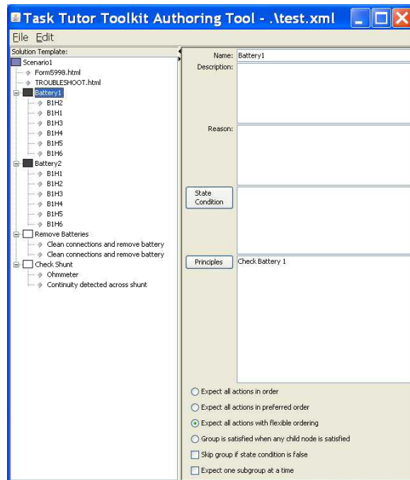
Figure 3: Solution template for the prototype scenario.
