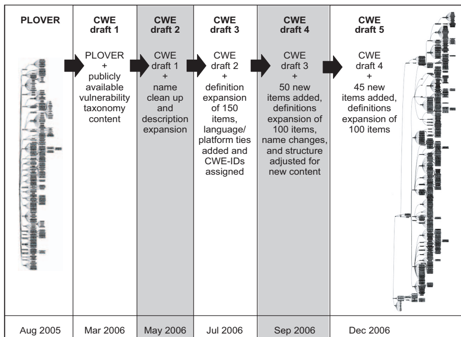
Figure 2: From PLOVER to CWE, Drafts 1-5
