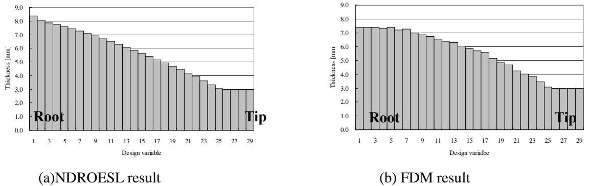
Fig. 11 Thickness distribution of the optimum models from NDROESL and FDM
