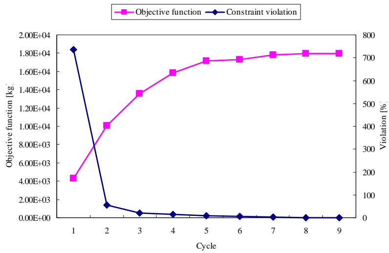
Fig. 17 History of nonlinear dynamic response structural optimization
