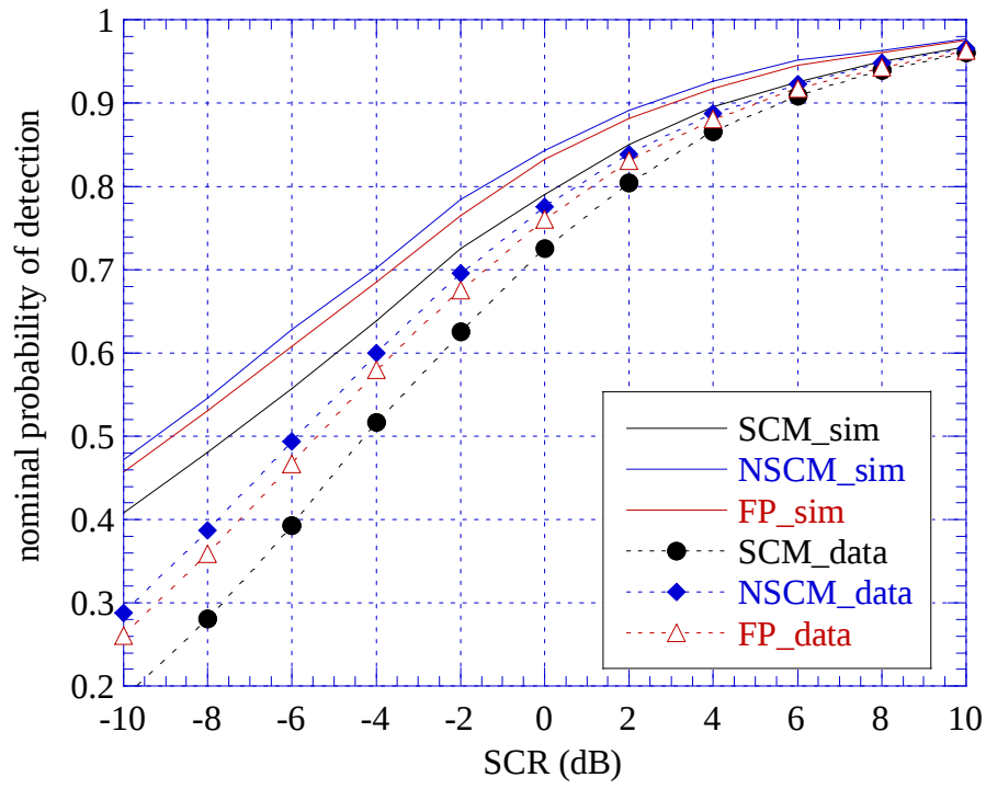
Fig. 40 – Probability of detection, N=8 , K=16 , P_{FA0}=10^{-2} , VV polarization.
