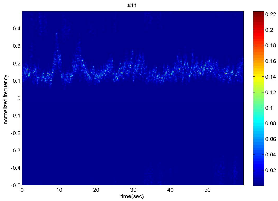
Fig. 20 – Spectrogram of the 11 th cell, HH data, 2 nd file.
