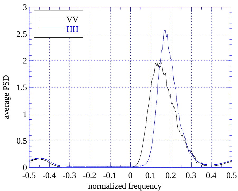
Fig. 12 – Average PSD of sea clutter, 3 rd file.
