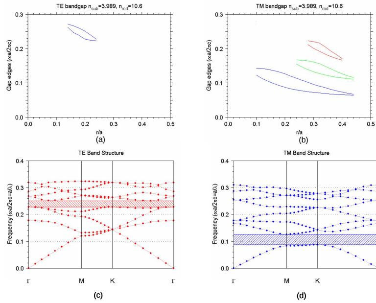
Fig. 6 Photonic bandgap for Type 2 photonic crystals (GaAs column in Ge slab): Gap maps at different r/a values for (a) TE and (b) TM polarizations; Bandgap plots at r/a=0.2 for (c) TE and (d) TM polarizations.
