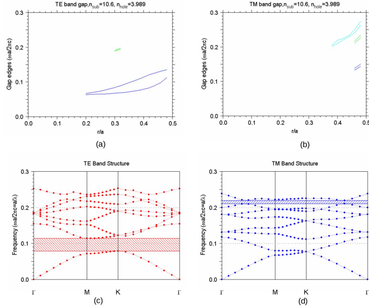
Fig. 5. Photonic bandgap for Type 1 photonic crystals (Ge column in GaAs slab): Gap maps at different r/a values for (a) TE and (b) TM polarizations; Bandgap plots at r/a=0.4 for (c) TE and (d) TM polarizations.
