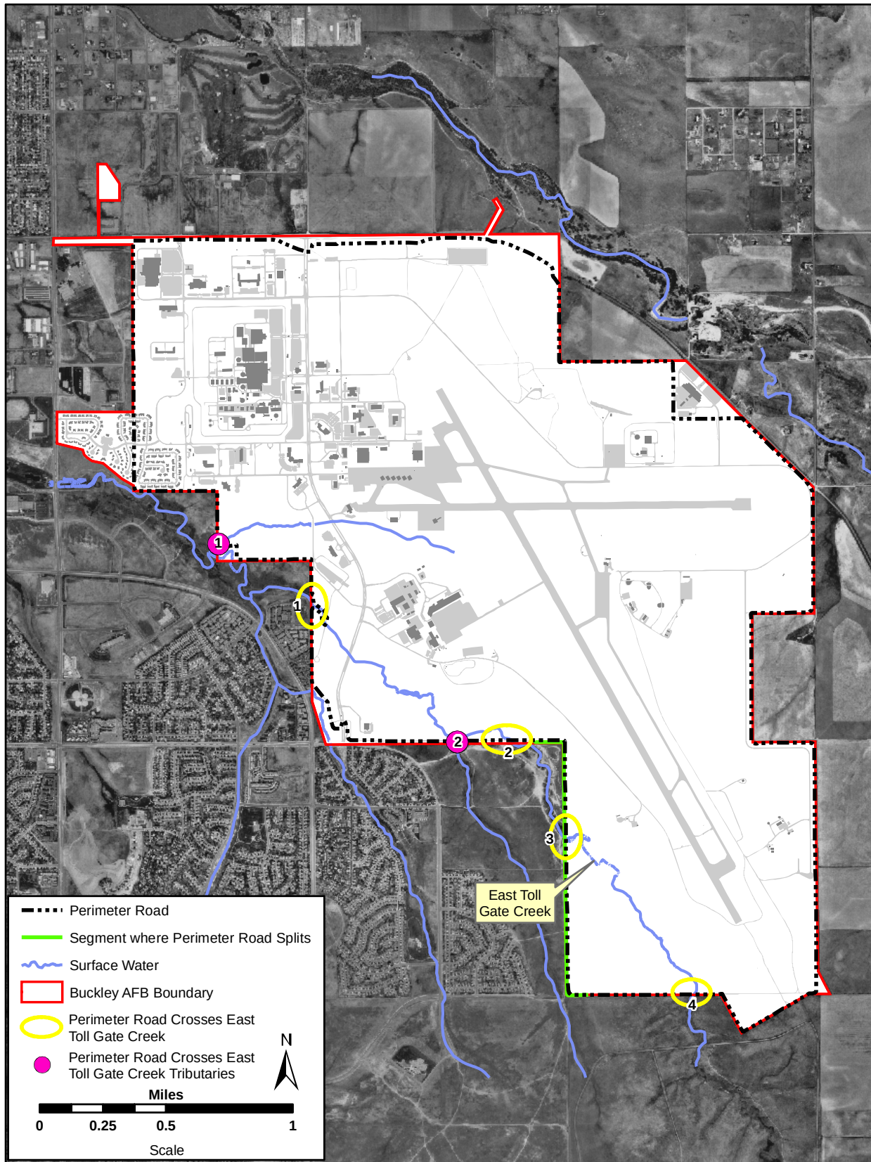
Figure 2-1. Existing Perimeter Road at Buckley AFB
