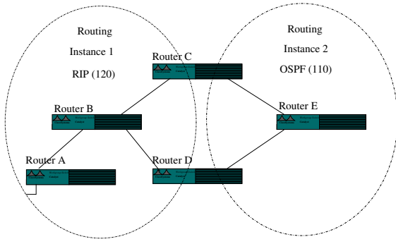
Fig. 5. Routers C and D are performing mutual route redistribution. The redistribution can result in persistent routing loops ( C-B-D-E-C ) for prefixes originated from the RIP domain or injected into the RIP domain (e.g., through router A )
