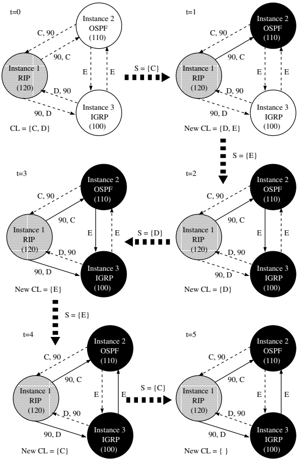
Fig. 15. Illustration of an activation sequence when the AD for C.1 and D.1 are set to 90. The redistributions converge to a cycle-free state.
