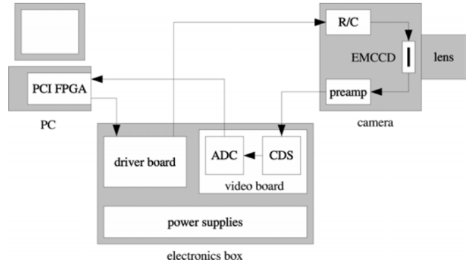
Fig. 6. Schematic showing the setup for the prototype EMCCD camera.
