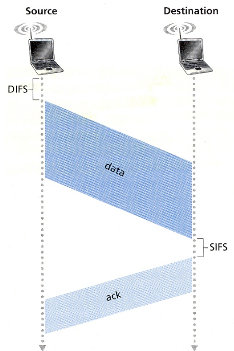
Figure 4. 802.11 Link-Layer Acknowledgements (Kurose, 2007:533)
