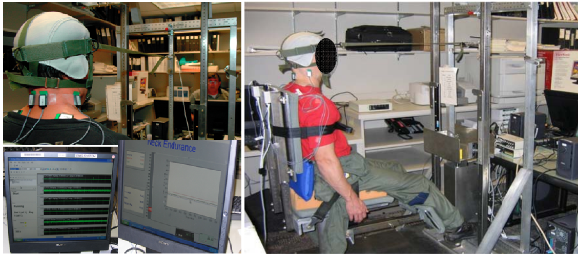
Figure 2. Neck Strength Test Fixture
