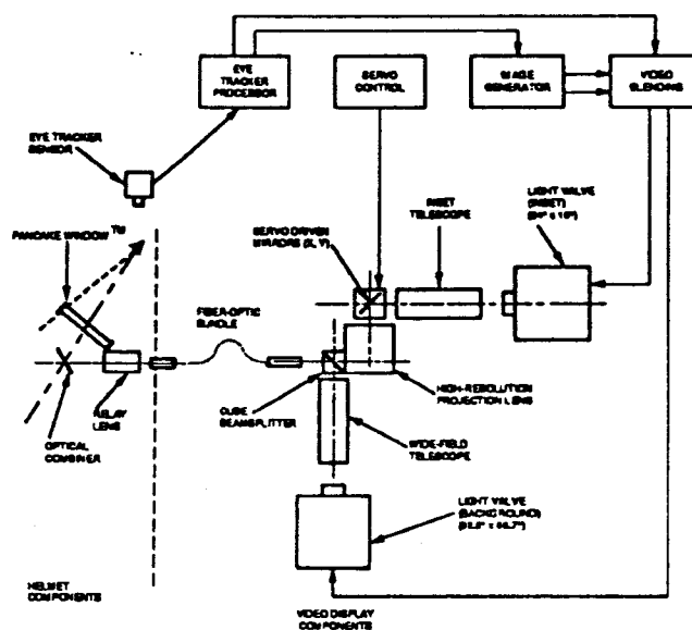
Figure 2. FOHMD/AOI Block Diagram
