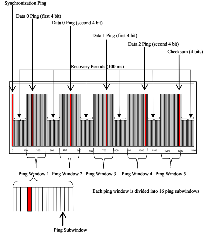
Fig. 5. Pulse Position Modulation of 2-Character Message Block
