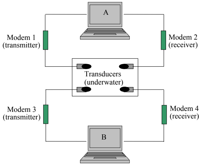
Fig. 2. Full-Duplex Test Bed Design
