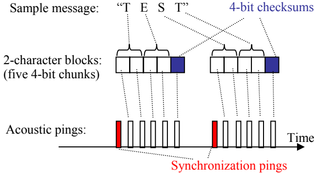
Fig. 4. Message Transission Schema of RBS-1 Modem
