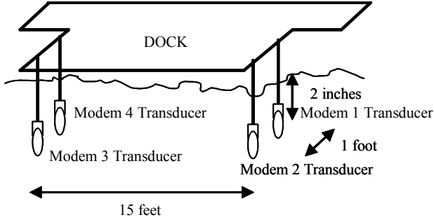
Fig. 3. Placement of Transducers in Lake Test
