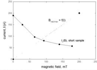
Fig. 3. The load line B_{r,\text{max}} = f(I) and I_c(B) curve of the YBCO tape used in the coil.
