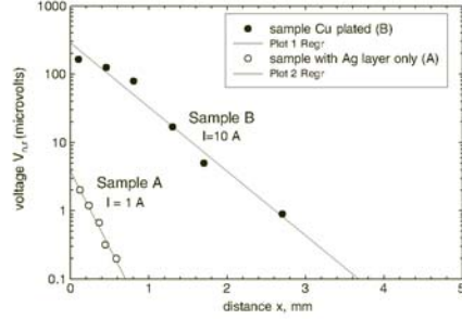
Figure 6. The current transfer voltage versus the distance of the measuring potential tap from the tape end for sample 1 (at 1 A) and for sample 2 (at 10 A). The straight lines are fits using linear regression.
