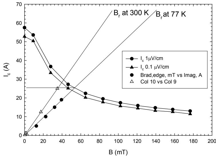
Figure 29.: The load line of the complete coil at 300K and 77 K
