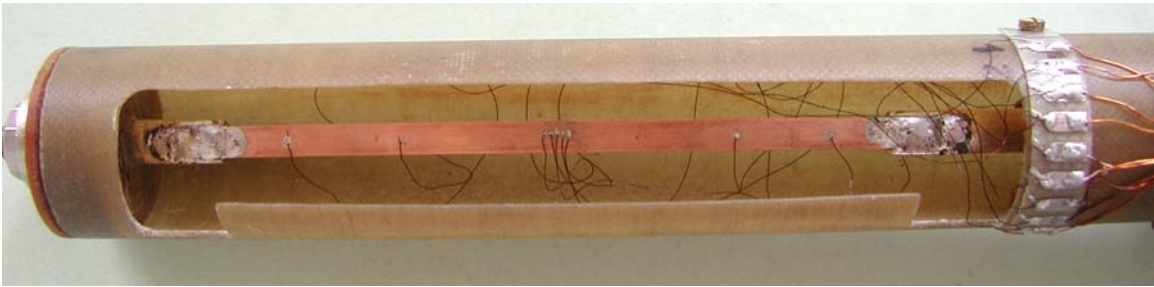
Figure 5.: The sample (tape) with the potential taps in the original, not twisted position
