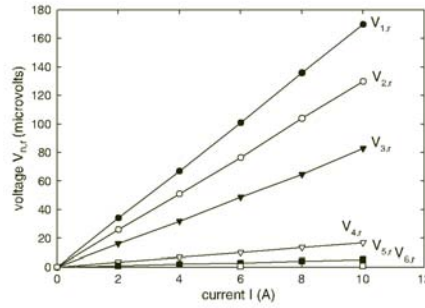
Figure 5. The current transfer voltage measured between tap n and the reference tap r , V_{n,r} , versus current I for sample 2 at 77 K.
