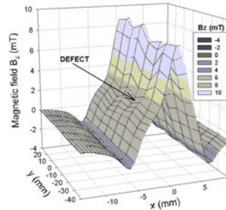
Fig. 3. Magnetic field map above sample P6, z_0 = 0.8 mm.
