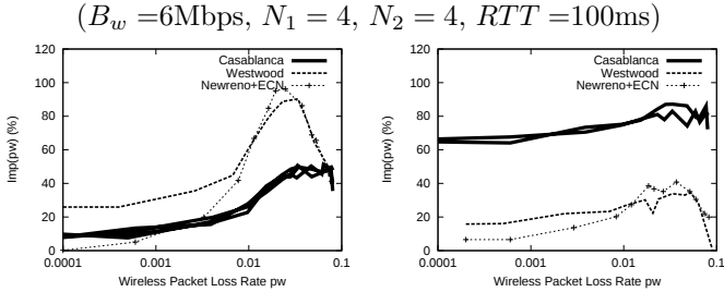
(a) No UDP Cross Traffic (b) 50% UDP Cross Traffic
