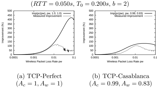
Figure 11: Imp and Measured Improvement
