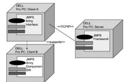
Figure 10: Deployment Diagram
