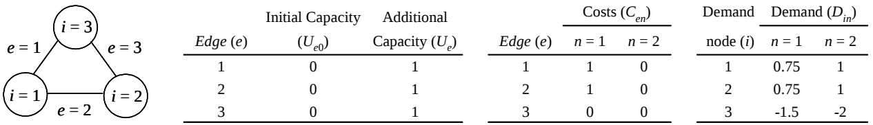
Figure 1: Data for an example in which the master problem of SV formulation has a fractional LP solution. The diagram on the left represents a distribution network with three edges that connect supply node 3 to demand nodes 1 and 2. The tables on the right contain data for a single-scenario, 2-stage problem instance, i.e., \mathcal{N} = \{1, 2\} ; here, U_{ehn} = U_e, \forall n \in \mathcal{N}, h \in \mathcal{P}_n .
