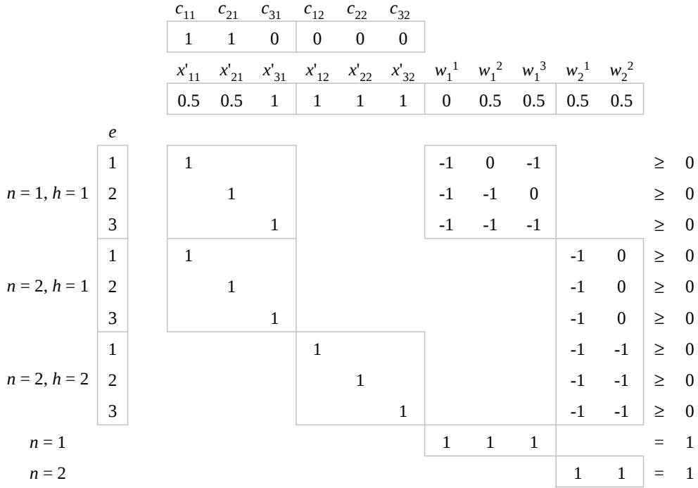
Figure 2: Constraint matrix and LP solution to the master problem of SV for the 2-stage single-scenario problem specified in figure 1. The solution is fractional.
