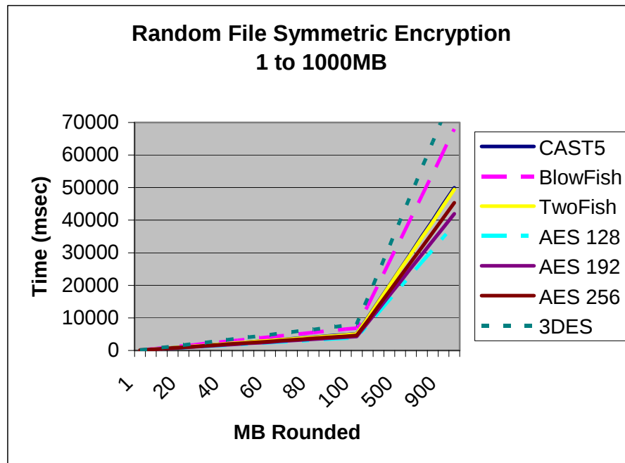
Figure 19. Symmetric Encryption for Random Files to 100MB
