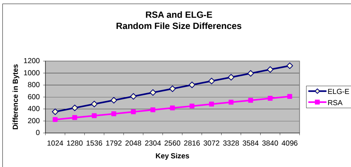
Figure 11. Comparison of Public Key File Size Differences
