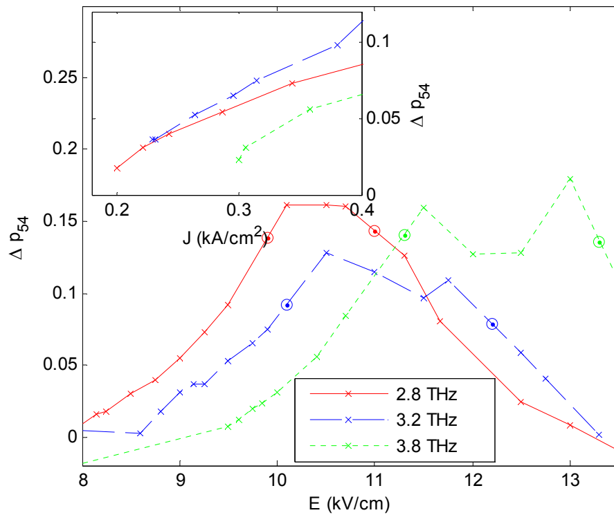
Fig. 3. Population difference between upper and lower laser level as a function of the applied field. The circles mark the positions of the anticrossings 5 - 2' and 5 - 1'. The inset shows \Delta p_{54} as a function of the current density close to the onset of inversion. The crosses mark the sampling points; the lines are guide to the eye.
