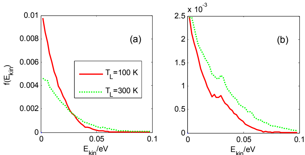
Fig. 10. Hole distribution functions of the (a) upper and (b) lower laser level as a function of the kinetic energy for an applied field of 43 kV/cm and lattice temperatures of 100 and 300 K.
