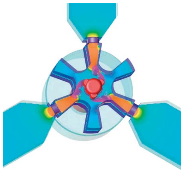
Shaped cathode in the A6-3 relativistic magnetron
