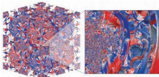
Figure B. Navier-Stokes free shear computed with an entropic lattice gas on a 1600^3 grid on BABBAGE (IBM P5+) using 2,048 processor elements at the NAVO MSRC. Nonlinear dynamics over disparate spatial scales is faithfully captured (inset).
