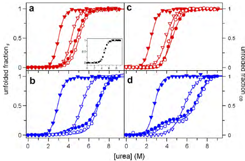
Fig. 4. Urea-induced unfolding (room temperature) of CopC monitored by fluorescence 356/320 nm ratio (a and b) and CD at 218 nm (c and d) for apo (a and c) and Cu II (b and d) forms at different pH conditions (filled triangles, pH 4; open triangles, pH 5; filled circles, pH 6; open circles, pH 7.5). Inset a: refolding data points for apo–CopC starting from 8 M urea conditions (open symbols) together with the direct unfolding data (filled symbols).
