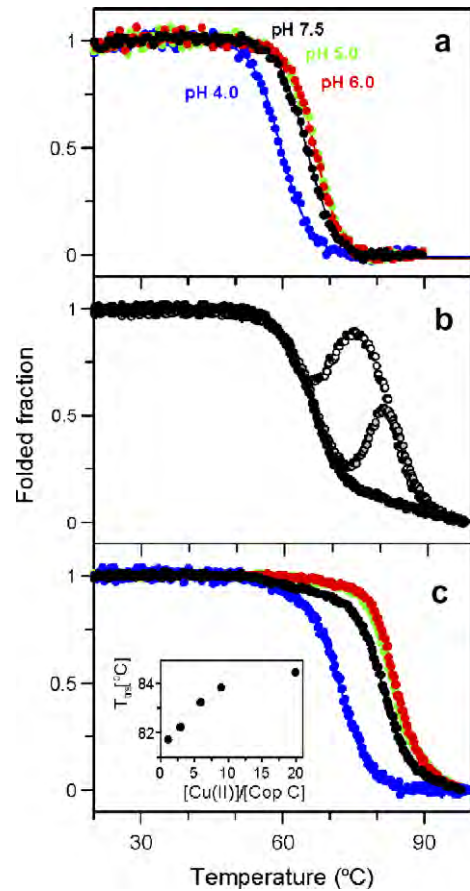
Fig. 5. Thermal unfolding monitored by CD for apo (a) and Cu II (c) forms at different pH values (pH 4, blue; pH 5, green; pH 6, red; pH 7.5, black). (b) Thermal unfolding curves for CopC in the presence of 1 equivalent of copper and 0.18 (white), 0.25 (grey), 0.5 (black) mM DTT (pH 7.5). Inset c: T trs for the major (second) transition versus excess Cu present in the solutions for Cu II –CopC at pH 7.5.
