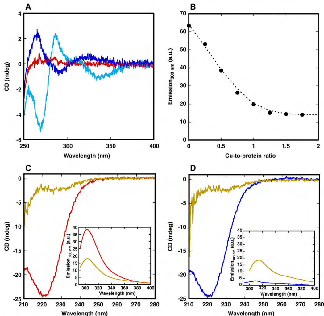
Fig. 2. (A) Near-UV CD of apo- (red) and holo-forms of CopZ: 1:2 (light blue, no DTT) and 1:1 (dark blue, 1 mM DTT) copper-to-protein complexes (pH 7.5, 20 °C). (B) Copper additions to apo-CopZ monitored by fluorescence changes at 303 nm (pH 7.5, 20 °C). (C) Far-UV CD spectra of folded (red; buffer, pH 7.5, 20 °C) and unfolded (gold; 5 M GuHCl, pH 7.5, 20 °C) forms of apo-CopZ. Inset C: fluorescence spectra of folded (red; buffer, pH 7.5, 20 °C) and unfolded (gold; 5 M GuHCl, pH 7.5, 20 °C) forms of apo-CopZ. (D) Far-UV CD spectra of folded (blue; buffer, pH 7.5, 20 °C) and unfolded (gold; 5 M GuHCl, pH 7.5, 20 °C) forms of holo-CopZ. Inset D: fluorescence spectra of folded (blue; buffer, pH 7.5, 20 °C) and unfolded (gold; 5 M GuHCl, pH 7.5, 20 °C) forms of holo-CopZ. Similar CD and emission spectra as in panels C and D were collected for folded and unfolded forms of apo- and holo-Atox1. Whereas the fluorescence decreases for the apo-forms upon unfolding, due to tyrosine exposure to solvent, the emission increases upon unfolding of the holo-forms as the fluorescence is quenched by the copper in the folded state.
