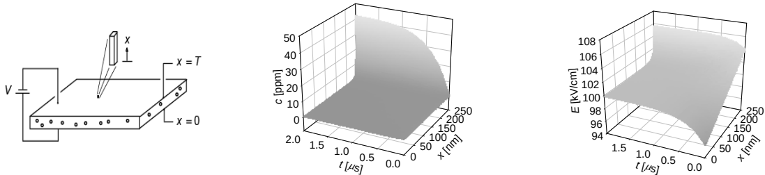
Fig. 1. Numerical solution (1-D) for BST film of thickness T : (left) geometry, (center) transient vacancy concentration c , and (right) electric field E (initial concentration c_0 = 0.5 ppm, applied voltage V = \phi_{x=0} = 2.5 V).
