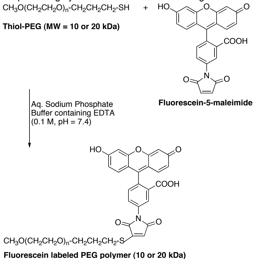
Scheme 1. General synthetic scheme to prepare fluorescein-labeled PEG polymers (10 and 20 kDa). The PEG-fluorescein (40 kDa) was obtained by analogous procedure. PEG-NH 2 was reacted with fluorescein succinimidyl ester at pH 8.0.
