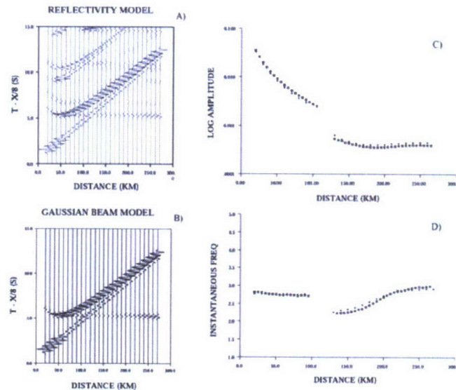
Figure 7 Synthetic seismograms and associated seismic attributes from the simple layer over a gradient model. A) Synthetic seismograms using the reflectivity method. B) Synthetic seismograms using the Gaussian beam method. C) Amplitude of the envelope of the first arriving pulse as a function of distance. Notice that there is a sudden drop in amplitudes near distances of 100 km. Results from Gaussian beam modeling (pluses) and those from reflectivity (squares) are similar. D) Instantaneous frequency of the first arrival pulse as a function of distance. Beyond distance of about 120 km, instantaneous frequency actually increases with increasing distance. Again, results from Gaussian beam modeling (pluses) and those from reflectivity (squares) are similar. The source pulse is a Gabor wavelet with a dominant frequency of 2.77 Hz. To isolate elastic effects of wave propagation, a constant Q value of 2000 was assumed (from Nowack and Stacy, 2002).
