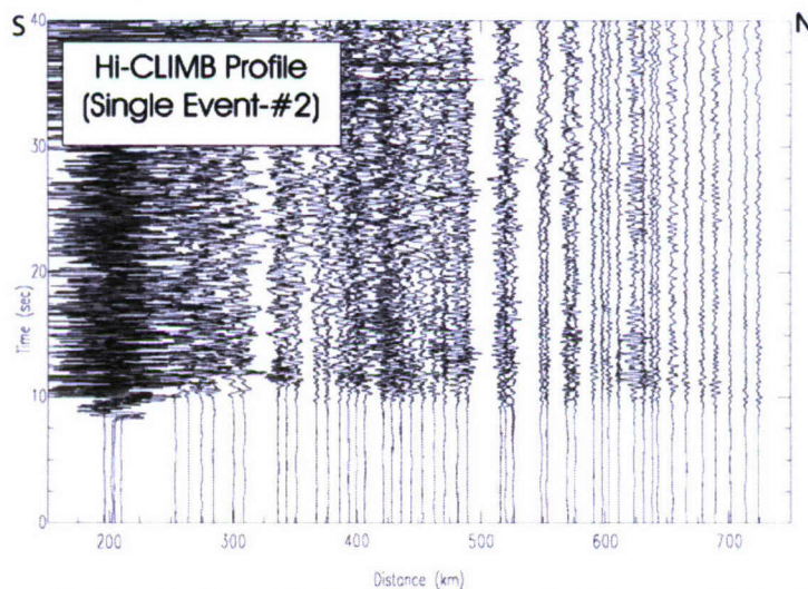
Figure 4. A second example of a seismic profile from a single event with a magnitude of 4.8 located directly south of the middle and northern sections of the Hi-CLIMB array. The P_n becomes the first arrival at distances beyond about 290 km. The time-scale is reduced by a wave speed of 8.0 km/s.
