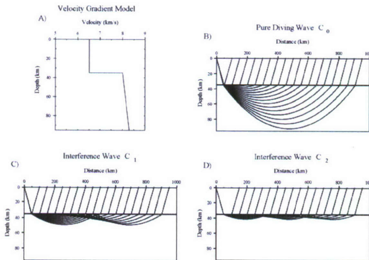
Figure 6. Illustration showing how a positive gradient in wave velocity beneath the Moho can affect the propagation of P_n . A) The model for P -wave speeds. The linear gradient beneath the Moho can simply arise from the spherical nature of the earth. B) Paths of the primary, diving rays (pure head waves are not shown). C) Paths of the first set of sub-Moho interference wave. D) Paths of the second set of sub-Moho interference wave (from Nowack and Stacy, 2002).
