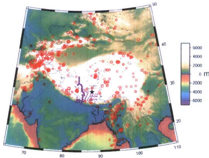
Figure 2. A color-coded topographic map, showing epicenters of large to moderate-sized earthquakes ( m_b 4.6 or above; open red circles) recorded by the Hi-CLIMB array (purple triangles). The asterisk marks the epicenter of a Tibetan earthquake ( m_b \sim 4.8 ) which serves as the seismic source of the preliminary profile shown in Figure 4.
