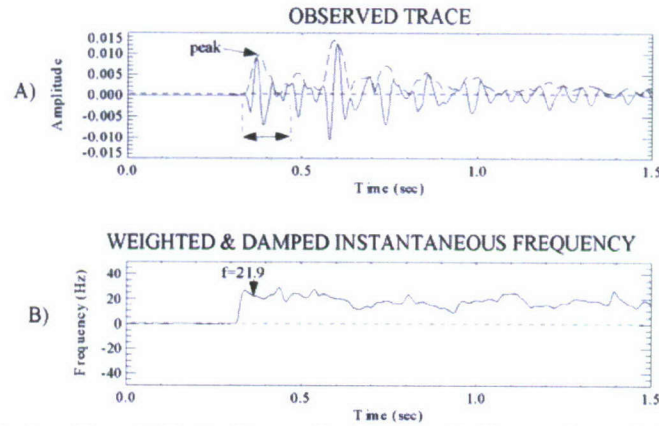
Figure 5. An example of extracting attributes from seismic data. A) Comparison of observed seismogram (solid trace) and its envelope calculated based on the Hilbert transform of data (dashed curve). The peak amplitude of the Hilbert envelope for the first pulse is marked. B) Damped and smoothed instantaneous frequency as a function of time (from Matheny and Nowack, 1995).
