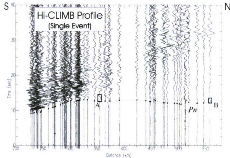
Figure 3. An example of seismic profile from a single event (marked by the star in Figure 2) recorded by central and northern portions of the Hi-CLIMB main array, showing clear arrivals of P_n (marked by the dotted curve) which become the first arrival at distances beyond about 325 km. Notice the dominant frequency of P_n actually can increase with distance: Compare signals marked by box A, about 0.5 Hz near 350 km; and box B, about 0.7 Hz near 550 km. Solid circles mark first arrivals at selected seismograms. The time-scale is reduced by a wave speed of 8.0 km/s.
