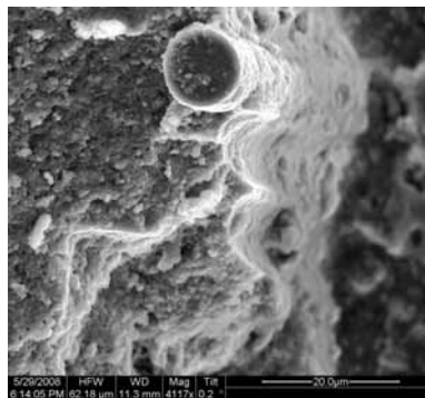
Figure A.452: Fracture surface of the N610/LaPO 4 /Al 2 O 3 -LaPO 4 -AlOCl specimen with 8ply HSW subjected to creep test at 48 MPa in steam at 1100 °C ( t_f = 2.06 h).
