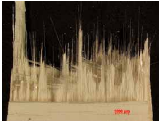
Figure B.54: Fracture surface of the N610/LaPO 4 /Al 2 O 3 specimen with 10ply 0°/90° uni-tape lay-up subjected tension to failure in laboratory air at 1100 °C.
