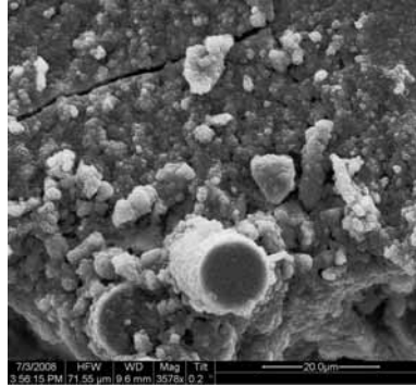
Figure A.166: Fracture surface of the N610/LaPO 4 /Al 2 O 3 specimen with 8ply HSW subjected to creep test at 32 MPa in air at 1100 °C ( t_f = 100\text{h} ).
