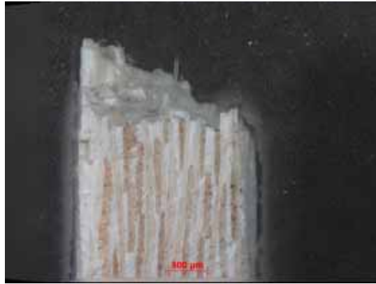
Figure B.217: Fracture surface of the N610/LaPO 4 /Al 2 O 3 -AlOCl specimen with 8ply HSW subjected subjected to creep test at 32 MPa in air at 1100 °C ( t_f > 100 h).
