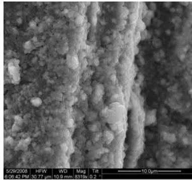
Figure A.451: Fracture surface of the N610/LaPO 4 /Al 2 O 3 -LaPO 4 -AlOCl specimen with 8ply HSW subjected to creep test at 48 MPa in steam at 1100 °C ( t_f = 2.06 h).
