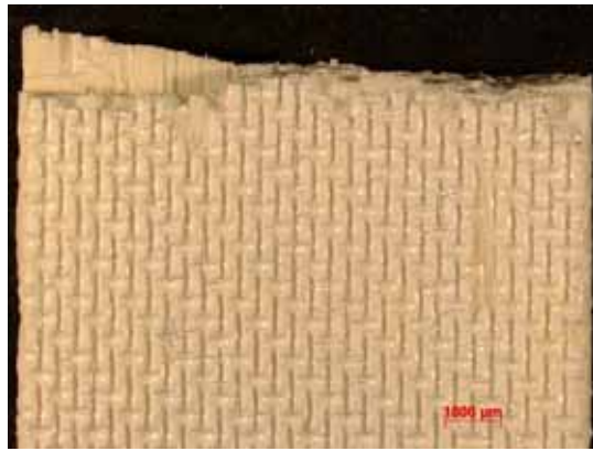
Figure B.180: Fracture surface of the N610/LaPO 4 /Al 2 O 3 specimen with 8ply HSW subjected subjected to creep test at 30 MPa in steam at 1100 °C ( t_f = 16.1 h).
