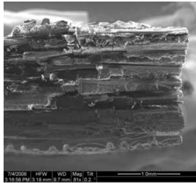
Figure A.226: Fracture surface of the N610/LaPO 4 /Al 2 O 3 specimen with 8ply HSW subjected to creep test at 72 MPa in steam at 1100 °C ( t_f = 2.24h ).
