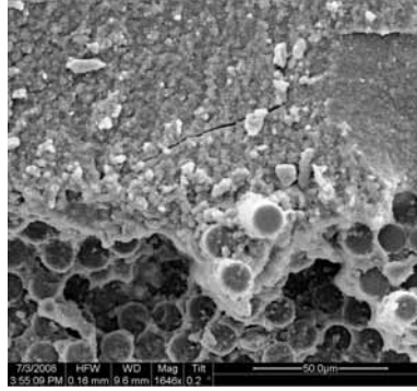
Figure A.165: Fracture surface of the N610/LaPO 4 /Al 2 O 3 specimen with 8ply HSW subjected to creep test at 32 MPa in air at 1100 °C ( t_f = 100\text{h} ).
