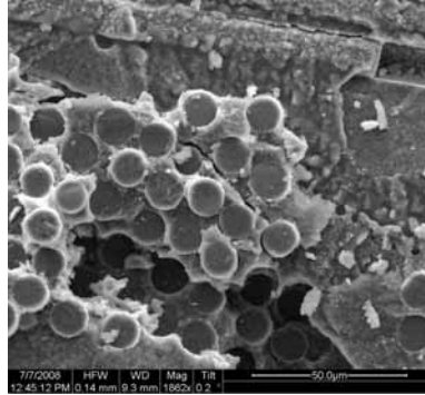
Figure A.370: Fracture surface of the N610/LaPO 4 /Al 2 O 3 -LaPO 4 -AlOCl specimen with 8ply HSW subjected to creep test at 32 MPa in air at 1100 °C ( t_f = 100\text{h} ).
