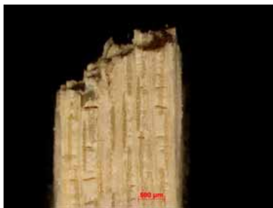
Figure B.230: Fracture surface of the N610/LaPO 4 /Al 2 O 3 -AlOCl specimen with 8ply HSW subjected subjected to creep test at 32 MPa in steam at 1100 °C ( t_f = 3.47 h).
