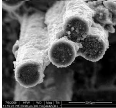
Figure A.273: Fracture surface of the N610/ \text{Al}_2\text{O}_3 specimen with 8ply HSW subjected to creep test at 30 MPa in steam at 1100 °C ( t_f = 16.1\text{h} ).
