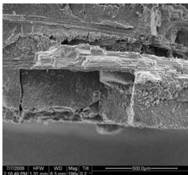
Figure A.403: Fracture surface of the N610/LaPO 4 /Al 2 O 3 -LaPO 4 -AlOCl specimen with 8ply HSW subjected to creep test at 32 MPa in steam at 1100 °C ( t_f = 3.47\text{h} ).
