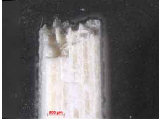
Figure B.43: Fracture surface of the N610/ \text{Al}_2\text{O}_3 - \text{LaPO}_4 specimen with 10ply 0^\circ/90^\circ uni-tape lay-up subjected to creep test at 25 MPa in steam at 1100 °C ( t_f = 40.1 h).
