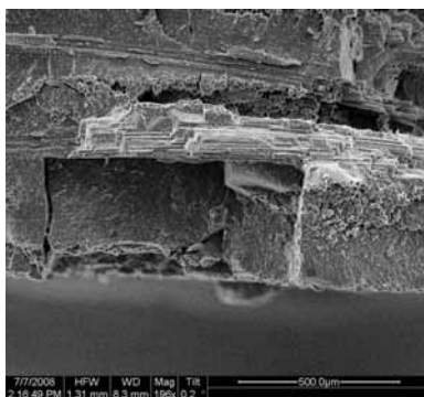
Figure A.402: Fracture surface of the N610/LaPO 4 /Al 2 O 3 -LaPO 4 -AlOCl specimen with 8ply HSW subjected to creep test at 32 MPa in steam at 1100 °C ( t_f = 3.47\text{h} ).
