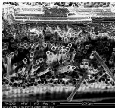
Figure A.227: Fracture surface of the N610/LaPO 4 /Al 2 O 3 specimen with 8ply HSW subjected to creep test at 72 MPa in steam at 1100 °C ( t_f = 2.24h ).
