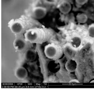
Figure A.61: Fracture surface of the N610/LaPO 4 /Al 2 O 3 specimen with 10ply 0°/90° uni-tape lay-up subjected to creep test at 85 MPa in air at 1100 °C ( t_f = 16.23\text{h} ).
