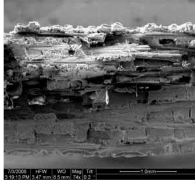
Figure A.141: Fracture surface of the N610/LaPO 4 /Al 2 O 3 specimen with 8ply HSW subjected to creep test at 32 MPa in air at 1100 °C ( t_f = 100\text{h} ).
