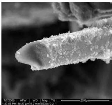
Figure A.397: Fracture surface of the N610/LaPO 4 /Al 2 O 3 -LaPO 4 -AlOCl specimen with 8ply HSW subjected to creep test at 32 MPa in air at 1100 °C ( t_f = 100h ).
