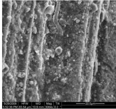
Figure A.450: Fracture surface of the N610/LaPO 4 /Al 2 O 3 -LaPO 4 -AlOCl specimen with 8ply HSW subjected to creep test at 48 MPa in steam at 1100 °C ( t_f = 2.06 h).
