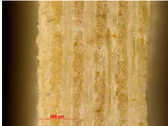
Figure B.1: Side view of the virgin N610/ \text{Al}_2\text{O}_3 - \text{LaPO}_4 specimen with 10ply 0^\circ/90^\circ uni-tape lay-up.
