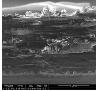
Figure A.225: Fracture surface of the N610/LaPO 4 /Al 2 O 3 specimen with 8ply HSW subjected to creep test at 72 MPa in steam at 1100 °C ( t_f = 2.24h ).
