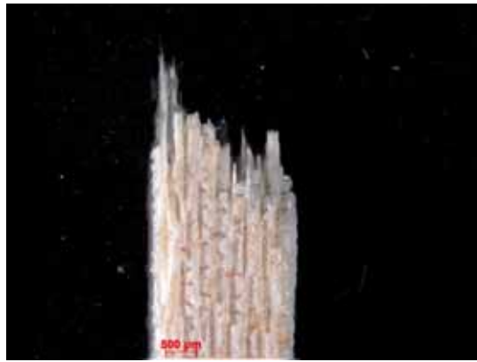
Figure B.111: Fracture surface of the N610/LaPO 4 /Al 2 O 3 specimen with 8ply HSW subjected tension to failure in laboratory air at 1100 °C.
