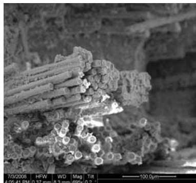
Figure A.167: Fracture surface of the N610/LaPO 4 /Al 2 O 3 specimen with 8ply HSW subjected to creep test at 32 MPa in air at 1100 °C ( t_f = 100\text{h} ).
