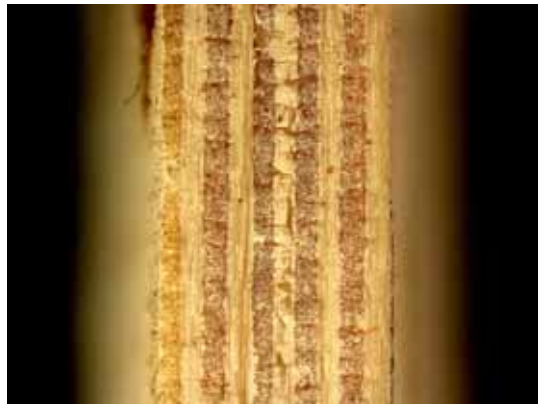
Figure B.48: Side view of the virgin N610/LaPO 4 /Al 2 O 3 specimen with 10ply 0°/90° uni-tape lay-up.
