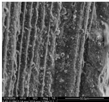
Figure A.449: Fracture surface of the N610/LaPO 4 /Al 2 O 3 -LaPO 4 -AlOCl specimen with 8ply HSW subjected to creep test at 48 MPa in steam at 1100 °C ( t_f = 2.06\text{h} ).
