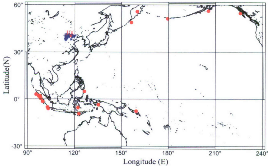
Figure 2. Map of event locations (red dots) and broadband stations (stars).
