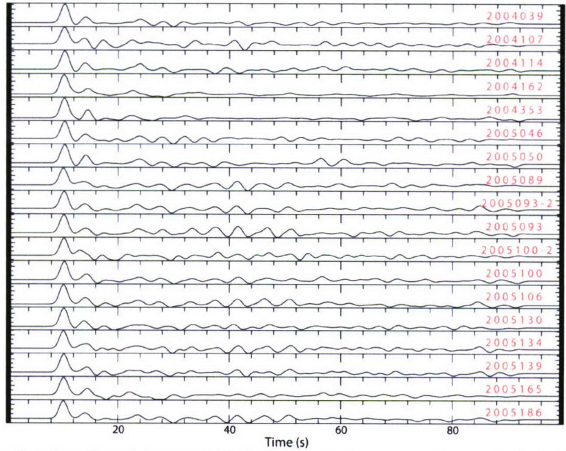
Figure 3. Receiver functions from 18 events with Gaussian window parameters \alpha = 1.0 , at station JIX.
