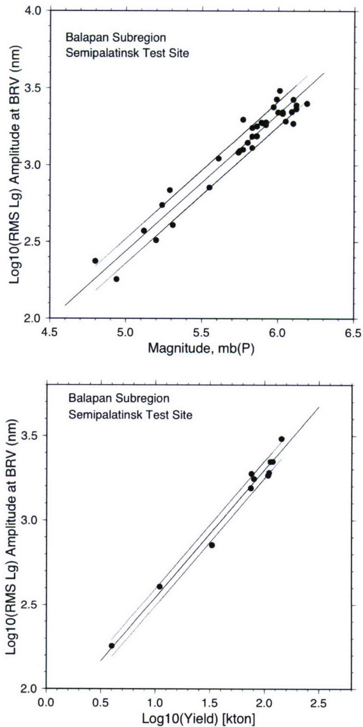
Figure 4. (Upper panel) Comparison of \log_{10}(\text{RMS Lg}) measurements in nm at BRV with body-wave magnitude mb(P). RMS Lg amplitudes are obtained from unfiltered data with a single gaussian window centered at an Lg group velocity of about 3.3 km/s. Solid line is a fitted slope of 0.89 and an orthogonal rms misfit of 0.060 magnitude units. The dotted lines correspond to \pm 2 S.D. (Lower panel) Comparison of \log_{10}(\text{RMS Lg}) measurements in nm at BRV with a reported yield in kilotons for 11 UNEs. Solid line is a fitted slope of 0.75 and an orthogonal rms misfit of 0.041 magnitude units. The dotted lines correspond to \pm 2 S.D.
