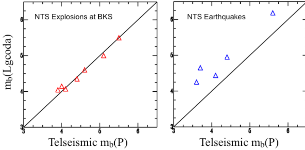
Figure 1. m_b(L_g\text{-coda}) at station BKS using the method of Mayeda et al. [2003] for selected NTS explosions are calibrated against the NEIC telseismic m_b (left) and correlate very well. However, the same path and site corrections applied to NTS earthquakes results in a bias of \sim 0.5\text{-}1 magnitude units (right).
