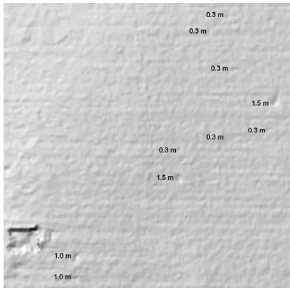
Ground returns surface model showing test craters.
