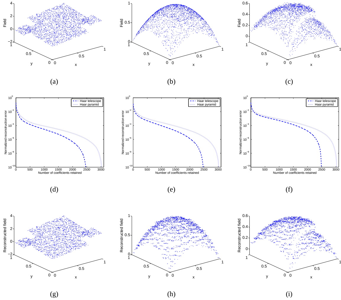
Fig. 9. Sample piecewise-constant (with a discontinuity) (a), quadratic (b), and noisy quadratic (with a discontinuity) (c) fields; approximation-error versus coefficient count curves (d),(e),(f); representative reconstructed fields (g), (h), (i)
