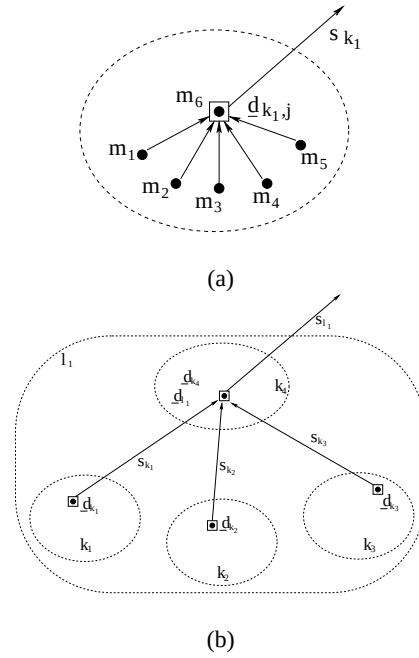
Fig. 2. Data flow (a) within a single cluster k_1 and (b) from clusterheads in k_1 through k_3 to the supercluster l_1 head in cluster k_4 .
