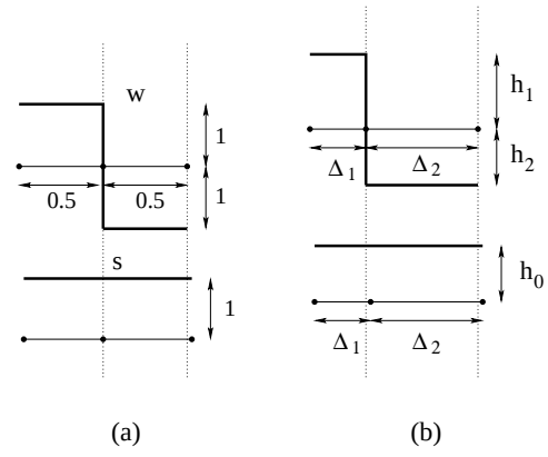
Fig. 5. (a) Regular, 1-D Haar wavelet ( W ) and scaling ( S ) basis functions and (b) corresponding matched pair telescope basis functions.
