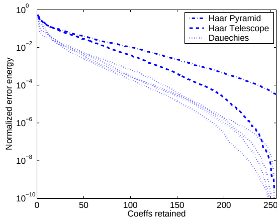
Fig. 8. Comparison of Haar Pyramid and Haar Telescope to D-2, D-4, D-6, and D-8 wavelets in a regular setting.
