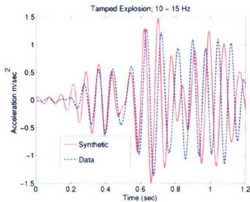
Figure 11. Spherical point explosion synthetics (red) and tamped explosion acceleration records (blue) at 710 m.
