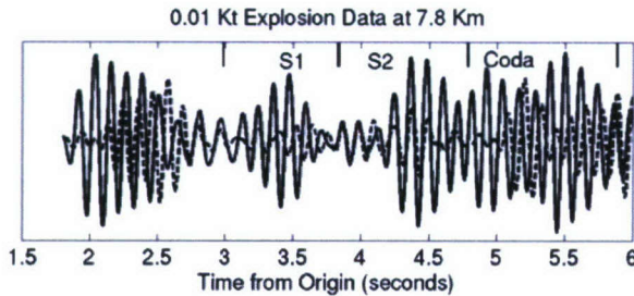
Figure 6. Overlain vertical (solid) and Hilbert transformed radial (dashed) velocity records of the 0.01 Kt explosion at 7.8 km, filtered from 5 to 10 Hz (above). The first and second S arrivals (labeled S1 and S2) and the coda are delimited by vertical bars along the upper plot boundary.
