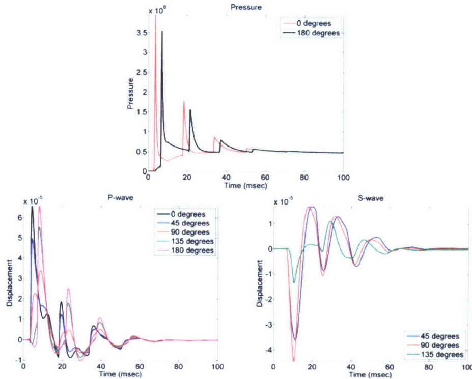
Figure 3. Cavity pressure at 0 (the offset direction) and 180 degrees (top) and far field P and S waves generated by the pressure function.
