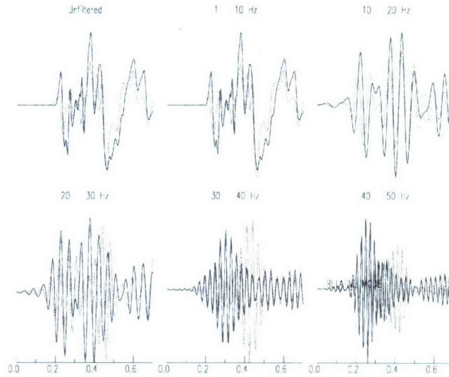
Figure 12. Vertical component records of the tamped (solid) explosion and the shallower partially decoupled explosion, at 145.4 and 163.2 m respectively. Initial P arrivals are aligned at 0.2 seconds.
