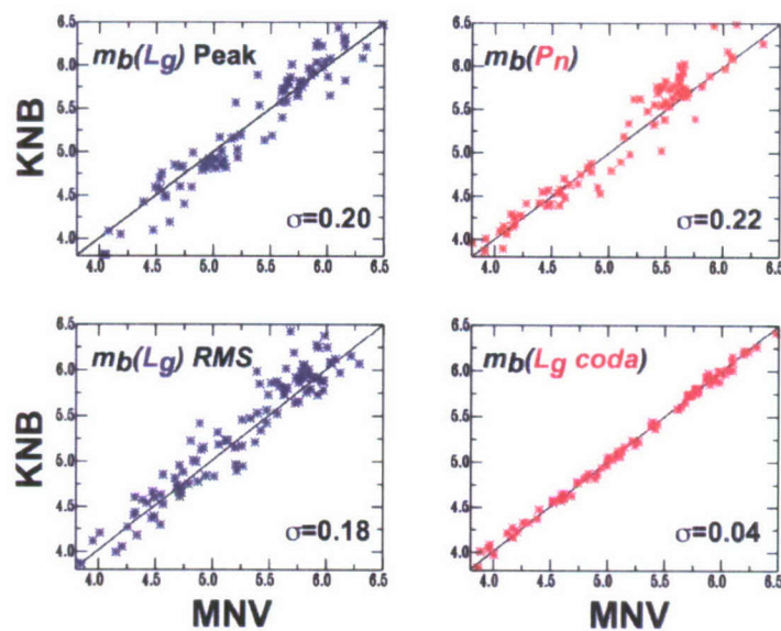
Figure 1. Interstation comparisons of magnitude at two near-regional stations, KNB ( \Delta \sim 250 km) and MNV ( \Delta \sim 200 km) (from Mayeda, 1993). Note that the scatter in the coda-derived m_b 's (lower right) are a factor of 4-to-5 times smaller than the conventional regional magnitude measures using direct P and L_g .
