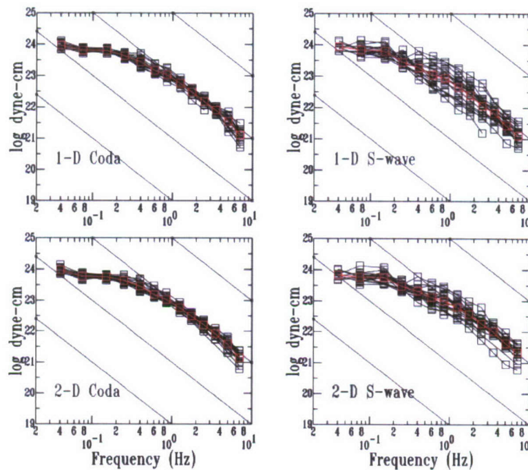
Figure 3. Absolute source spectra (moment-rate spectra) for the M_w 5.0 Napa earthquake of September 3, 2000. Top two panels show results assuming a one-dimensional (1-D), radially symmetric path corrections for coda and direct waves. Bottom panels show results using spatially varying two-dimensional (2-D) Q . Black lines represent individual station spectra, and red lines represent the average. Stations are situated at a variety of azimuths and range between a few tens of kilometers to over 400 km (from Mayeda et al, 2005). Notice that the coda-derived source spectra are remarkably stable in comparison with direct S and L_g spectra.
