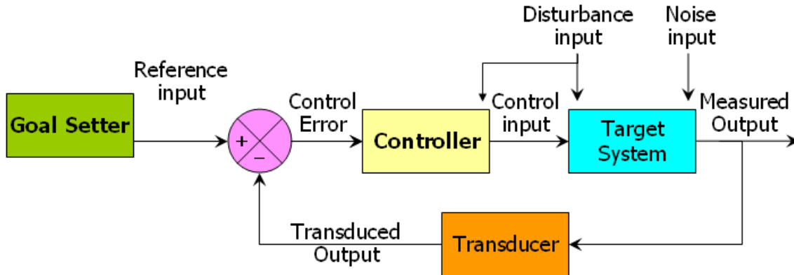
Figure 12: A Linear feedback-control system.
