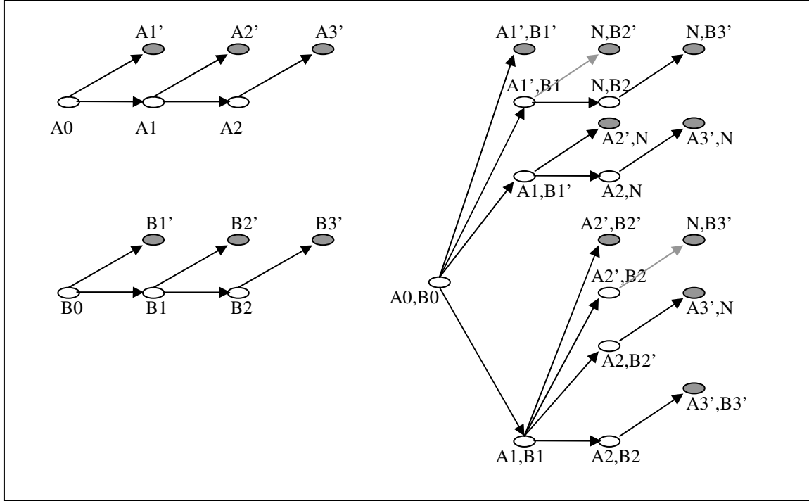
Figure 16: Combining the predictions of two independent task request events.
