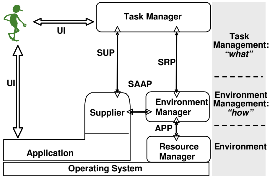
Figure 4: A component and connector view of the Aura Software Architecture.
