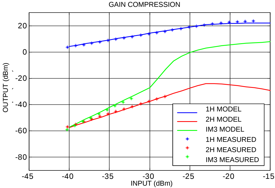
Figure 88. SHF amplifier gain curves.
