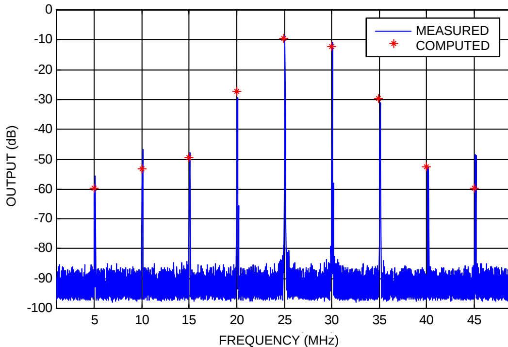
Figure 84. Mixer output spectrum IF range.
