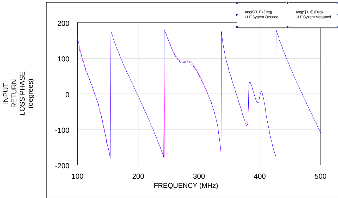
Figure 71. UHF system input return loss phase comparison.
