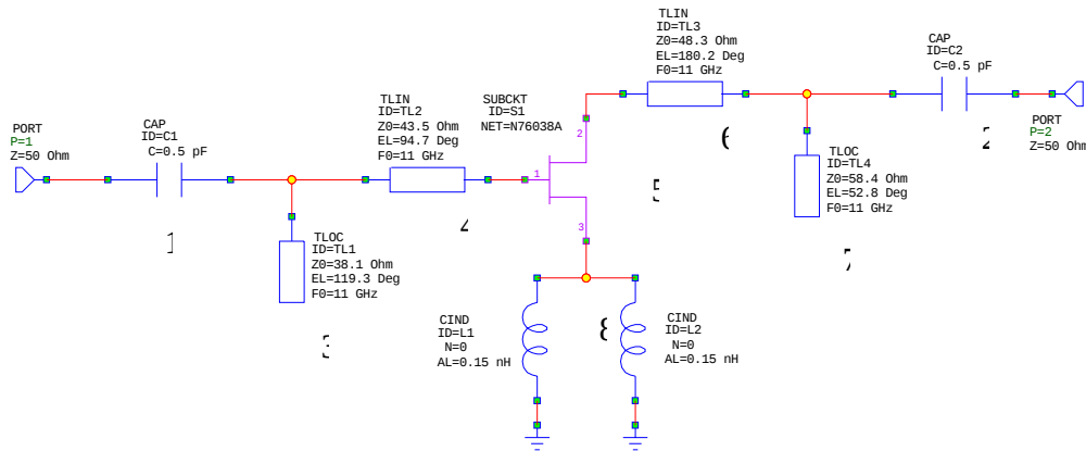
Figure 35. LNA schematic.
