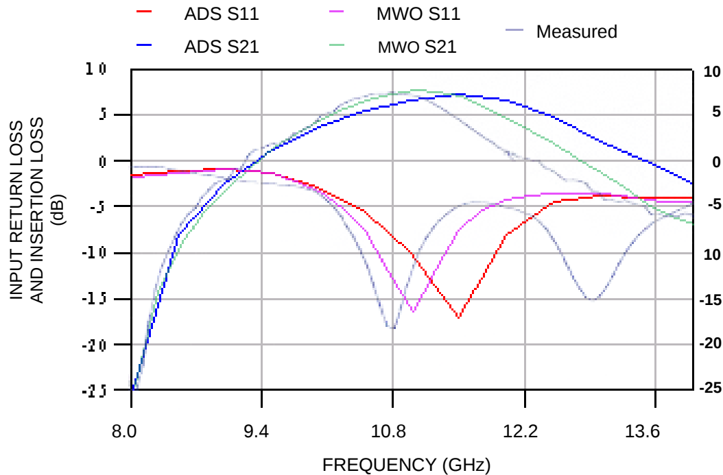
Figure 36. LNA S-parameters.
