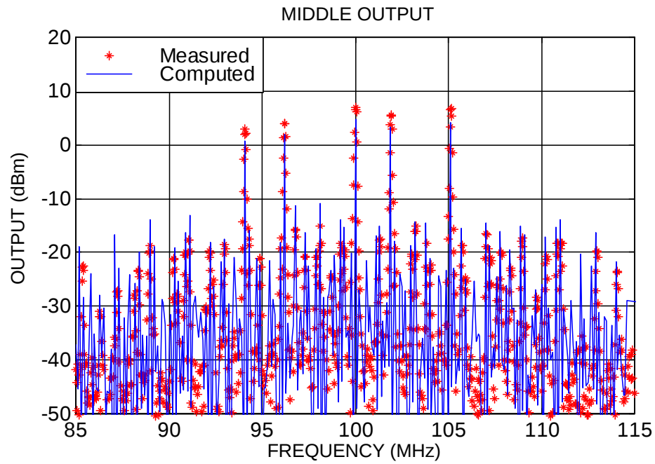
Figure 61. LNA output spectrum middle drive.
