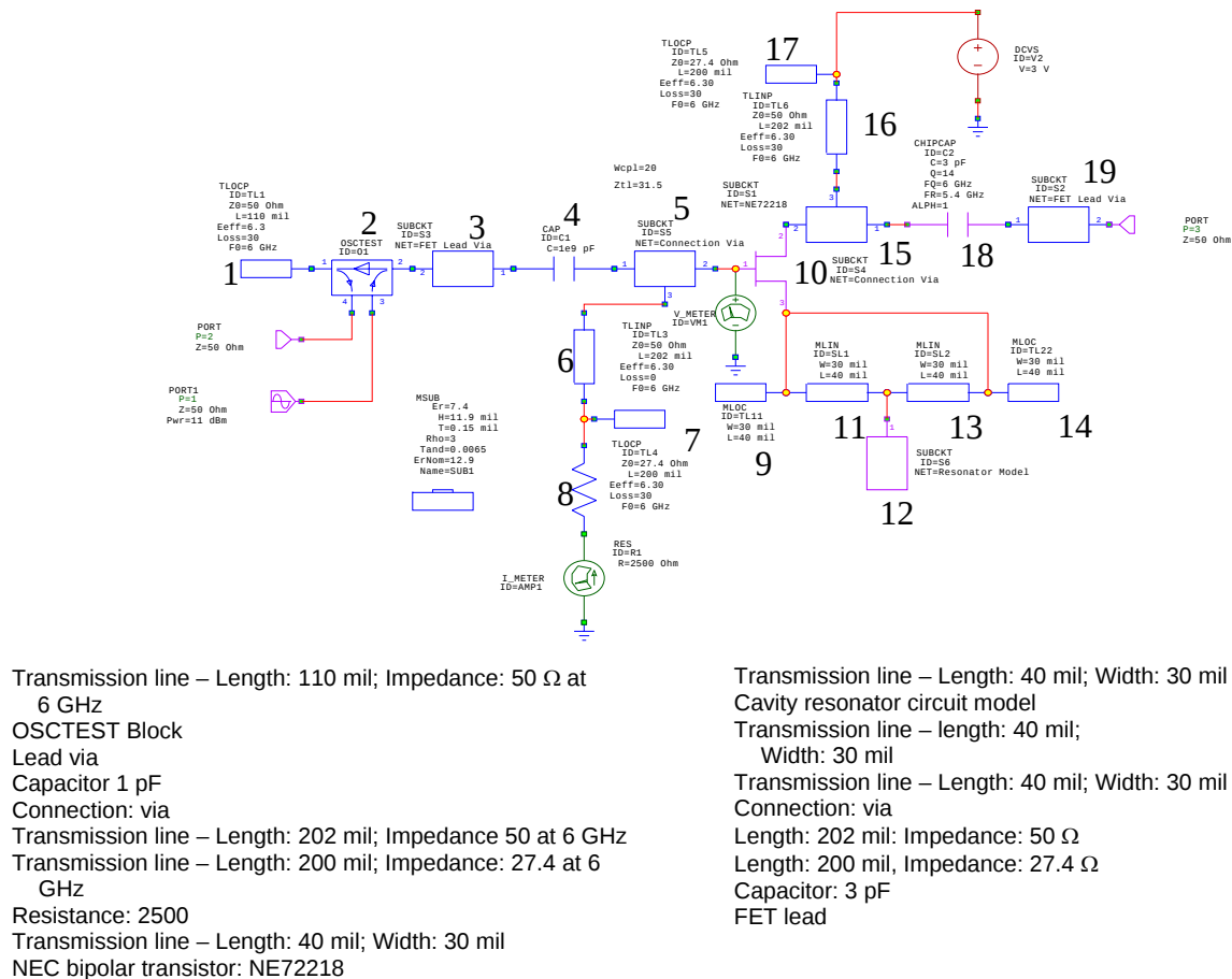
Figure 55. Tunable FET oscillator schematic.
