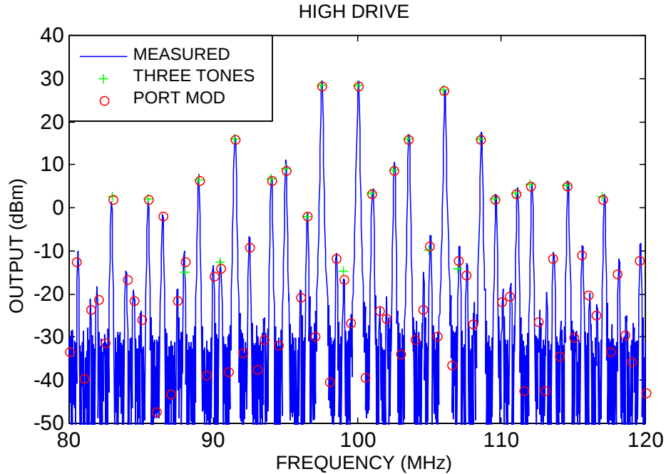
Figure 80. Power amplifier output spectrum high drive.
