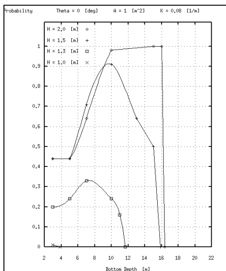
Figure 5 Detection probabilities for 1-m 2 circular cylinders of various heights, using a 0-degree scanner nadir angle on a 4m x 4m sounding grid; K=0.08 \text{ m}^{-1} .
