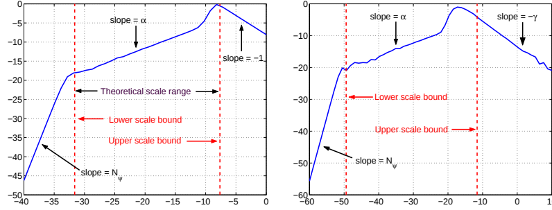
Figure 2: SCALING REGION AND CUTOFF SCALES: Choosing the scale too small, the resolution is fine enough for the wavelet to analyze the individual exponentials that form the estimator \hat{\phi} . According to section 4.4.1 the wavelet coefficients decay (at least) with exponent N_\psi . Choosing the scale too large, the estimator samples the body instead of the tail of the distribution; thus, the wavelet coefficients adhere to a powerlaw with exponent \lambda^- .
