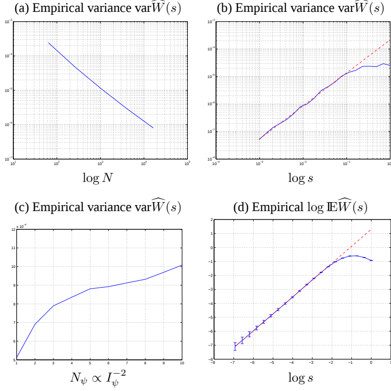
Figure 1: Experimental verification of expressions (50) and (51). (a)–(c): Empirical estimates of \widehat{\text{var}}\widehat{W}(s) estimated over a set of 100 independent realizations of \alpha -stable processes of length N . Evolution of \widehat{\text{var}}\widehat{W}(s) is plotted as a function of: (a) \log N ( \alpha = 1.2 , N_\psi = 4 , s = 0.0087 ); (b) \log s ( \alpha = 1.2 , N_\psi = 4 , N = 2^{14} ); (c) N_\psi ( \alpha = 1.2 , s = 0.0087 , N = 2^{14} ). (d) Empirical estimation of \log \mathbb{E}\widehat{W}(s) versus \log s . The error bars correspond to the standard deviation of \log \widehat{W}(s) . The dashed line materializes the theoretical law \log \mathbb{E}\widehat{W}(s) = \alpha \cdot \log(s) + C' ( \alpha = 1.2 , N_\psi = 4 , N = 2^{14} ).
