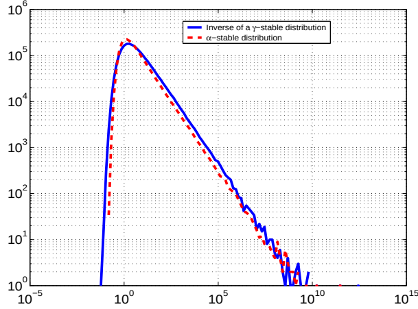
Figure 3: Empirical distributions of the random variables Y = X^{-1} and Z , where X follows a Gamma law with \gamma = 0.6 , and Z follows a stable law with \alpha = 0.6 and \beta = 1 . For both cases, \lambda^+ = \alpha = \gamma . Axis are in logarithmic scale.
