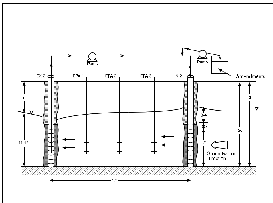
Figure 1: Process Diagram [1]
