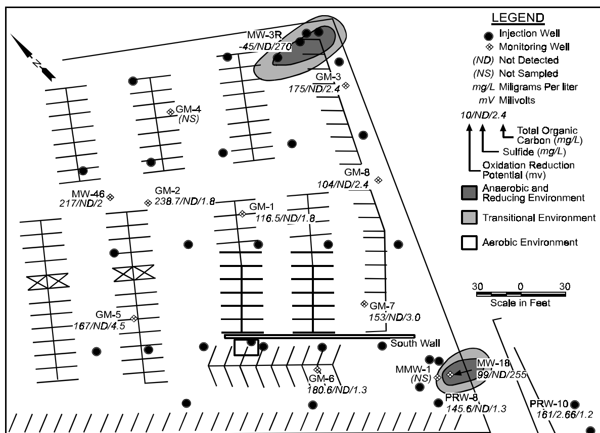
Figure 3: Distribution of Groundwater Indicator Parameters, Baseline Conditions, January 1997 [2,8]
