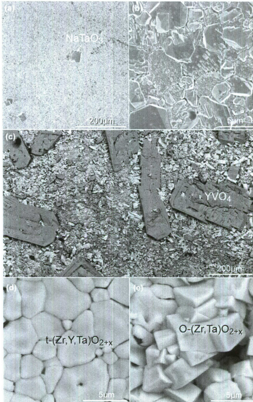
Fig. 14: SEM views of the surface of 16Y+16Ta samples after 75h exposure to \text{Na}_2\text{SO}_4 -30mole% \text{NaVO}_3 melts at 900^\circ\text{C} in air (a,b) and in \text{SO}_3/\text{SO}_2+\text{O}_2 (c-e). The surface in (a) contains a few relatively large faceted crystallites of \text{NaTaO}_3 , with no significant amount of depletion or other reaction products (b). The more aggressive environment leads to the formation of \text{YVO}_4 (c), with a slightly depleted tetragonal underlayer (d), \sim 25\mu\text{m} thick, and clusters of highly faceted orthorhombic (\text{Zr,Ta})\text{O}_{2+x} (e).
