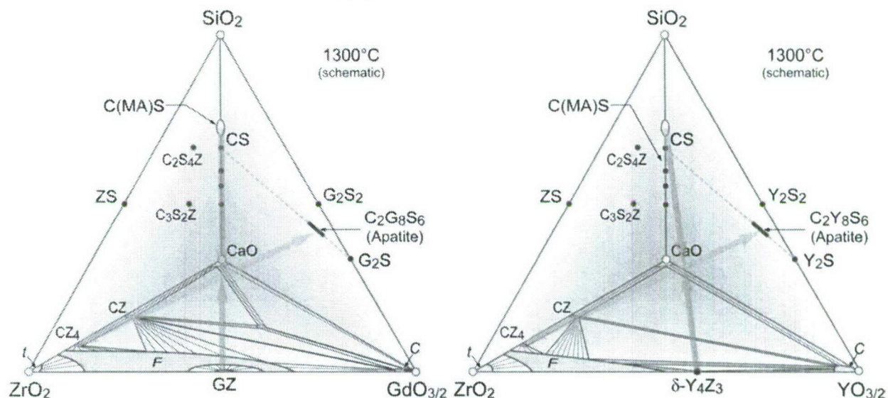
Fig. 4. Schematic comparison of the phases involved when CMAS reacts with the pyrochlore zirconate Gd 2 Zr 2 O 7 (a) and the \delta -phase zirconate Y 4 Zr 3 O 12 (b). The primary crystallization product is an oxyapatite of nominal composition Ca 2 (Gd/Y) 8 (SiO 4 ) 6 O 2 . In the ideal scenario the rest of the ingredients are combined in a (Zr,Ca) solution with the fluorite or the CaZr 4 O 9 structure. The MgO and AlO 1.5 in CMAS are ignored as a first approximation because they combine independently to form a separate spinel phase and minor other silicates.
