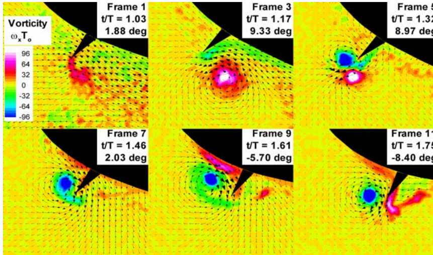
Figure 21: Sample PIV output from roll test
