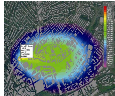
Figure 5 - Virtual battlespace
