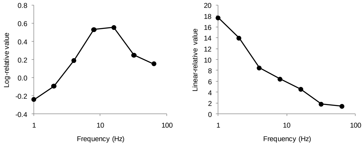
Figure 6. Log and linear dc level measures derived from relative probe threshold versus phase curves, averaged over two observers.
