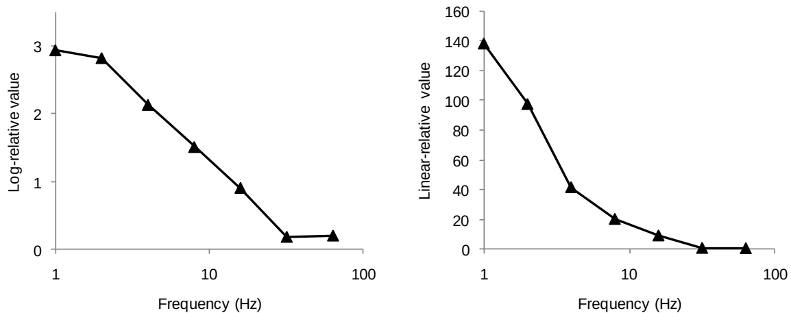
Figure 7. Log and linear peak-to-trough measures derived from relative probe threshold versus phase curves, averaged over two observers.
