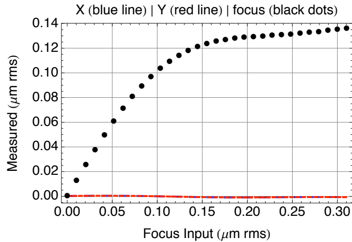
Figure 5. Measured Zernike coefficients for tilt and focus versus input focus for a 4 sub-aperture Shack-Hartmann sensor in the absence of noise.
