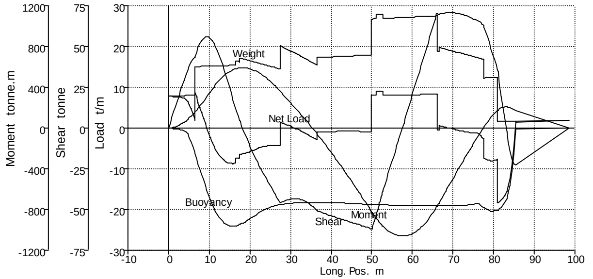
Figure A-25 Intact Logitudinal Load, Shear, and Bending Moment Diagram
