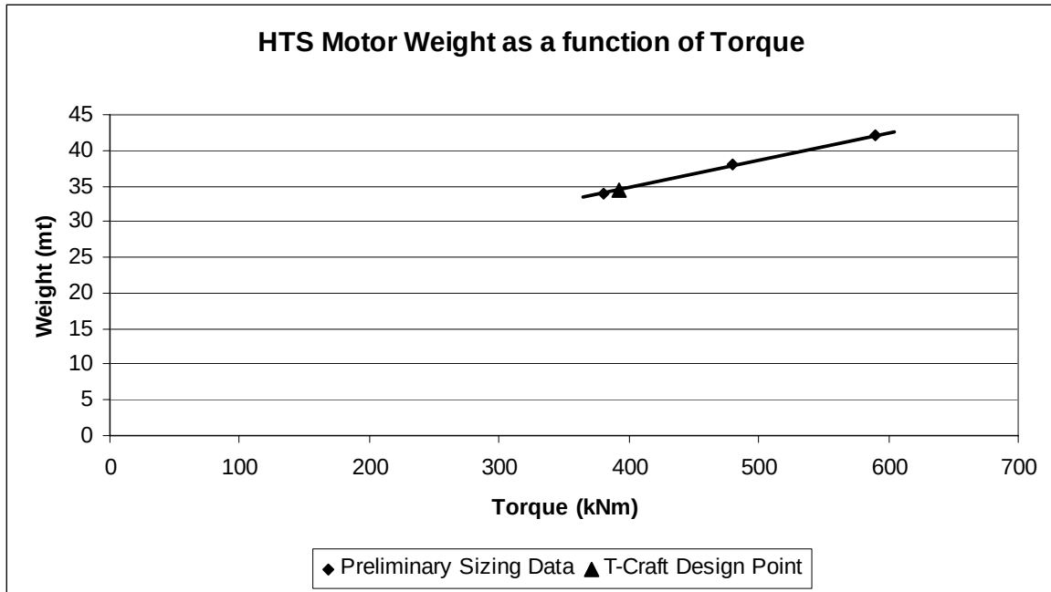
Figure 17: High Temperature Superconductor Motor Weight (data provided by American Superconductor)
