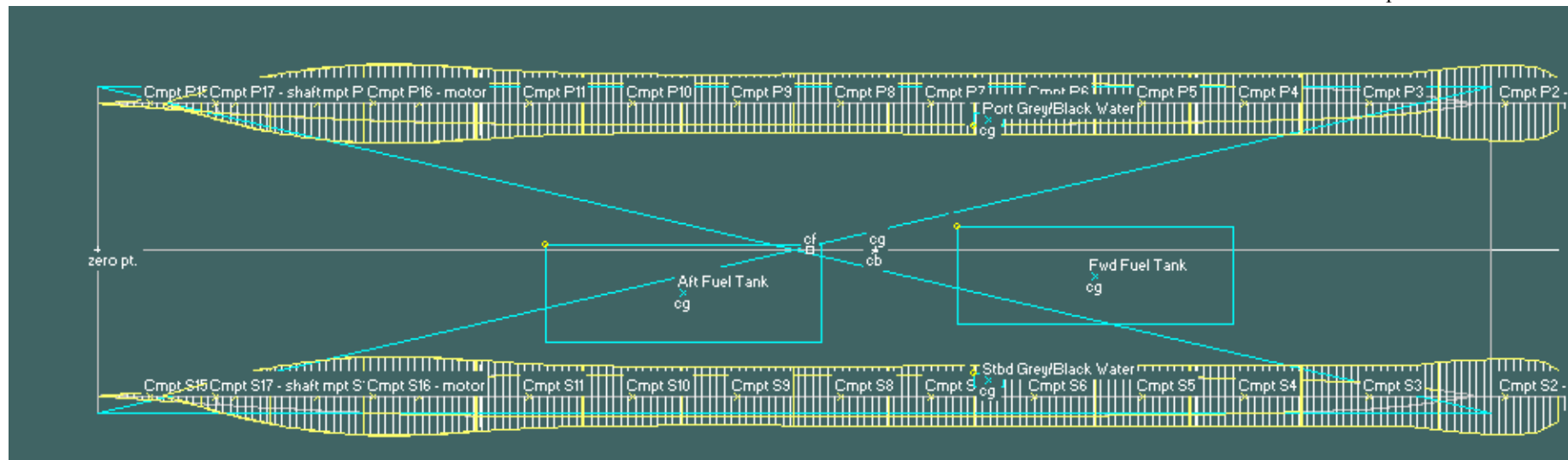
Figure A-19 Hydromax Plan - Tanks & Compartments – Fully Loaded Equilibrium Condition
