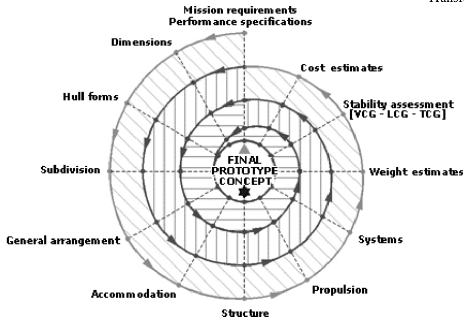
Figure 3: Design Spiral
