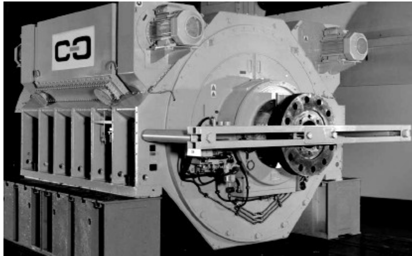
Figure 9 - Convertteam Advanced Induction Motor (Convertteam, 2006)
