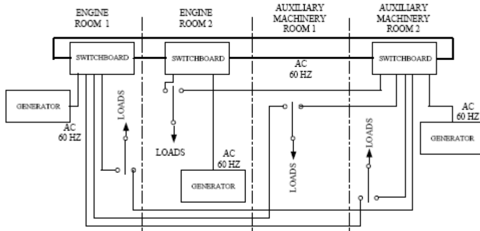
Figure 2 - AC Radial Distribution (Hegner & Desai, 2002, p. 336)
