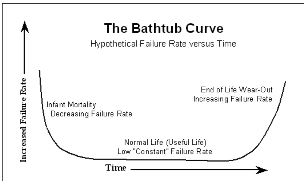
Figure 6 - The Bathtub Curve (Wilkins, 2002)
