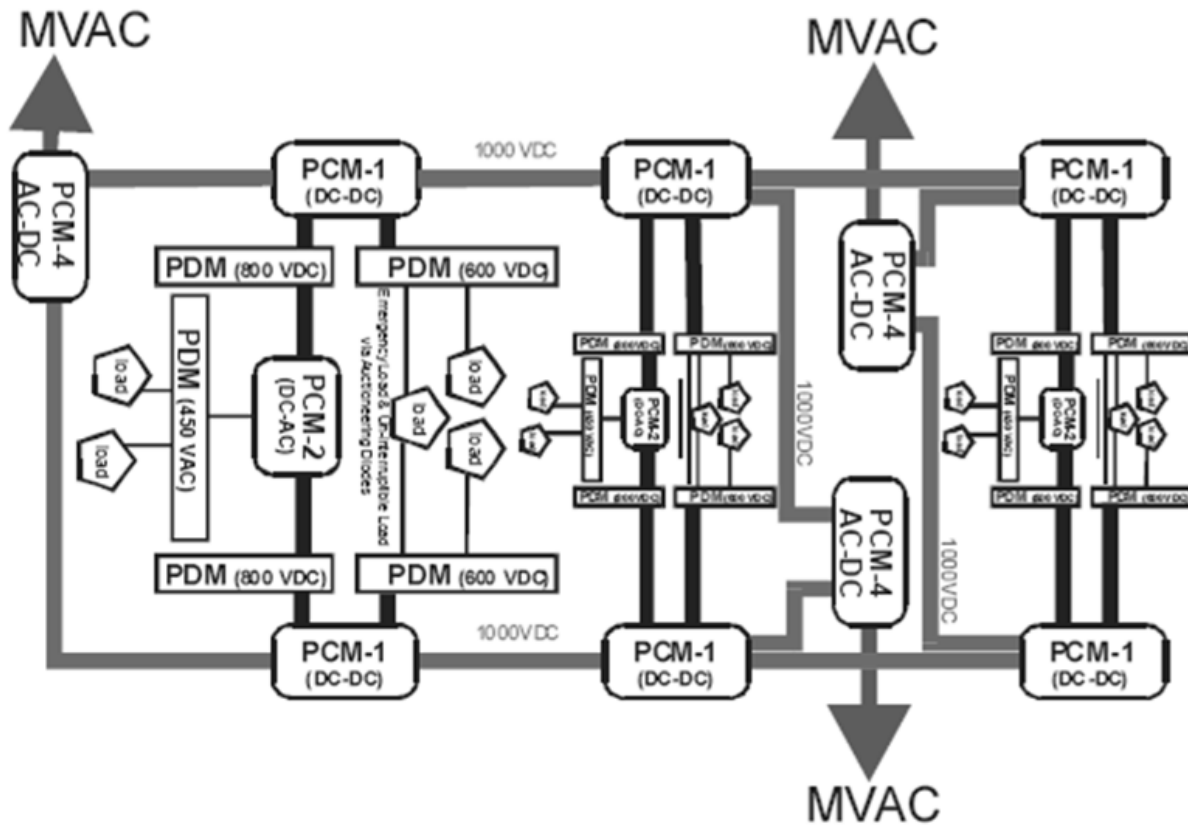
Figure 4 - Current Generation IFTP System (Doerry, 2007, p. 25)
