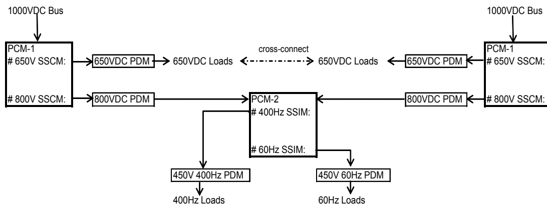
Figure 11 - Zonal IPS Architecture
