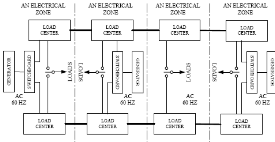
Figure 3 - AC ZED (Hegner & Desai, 2002, p. 337)
