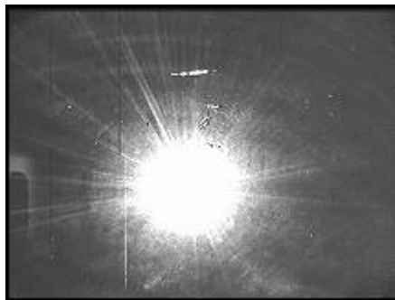
Figure 1.2-1. MWIR sensor that is jammed by a high flux collimated source.(Norman, 2006)
