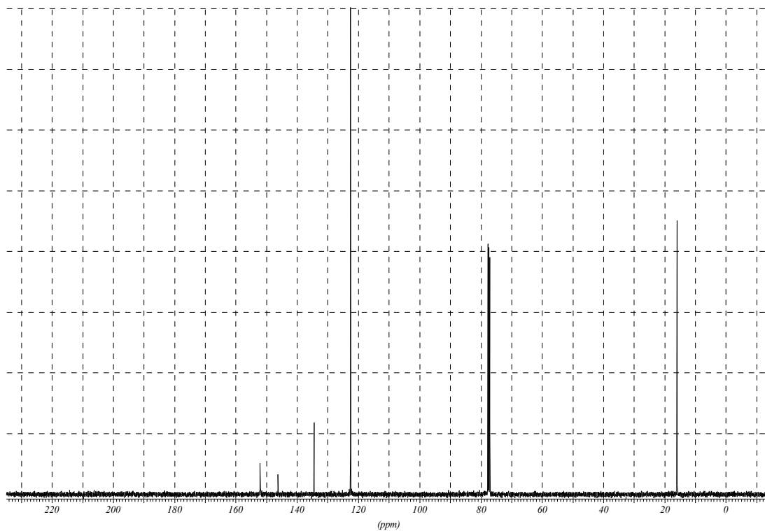
13 C NMR of Trinitrotoluene Sample
