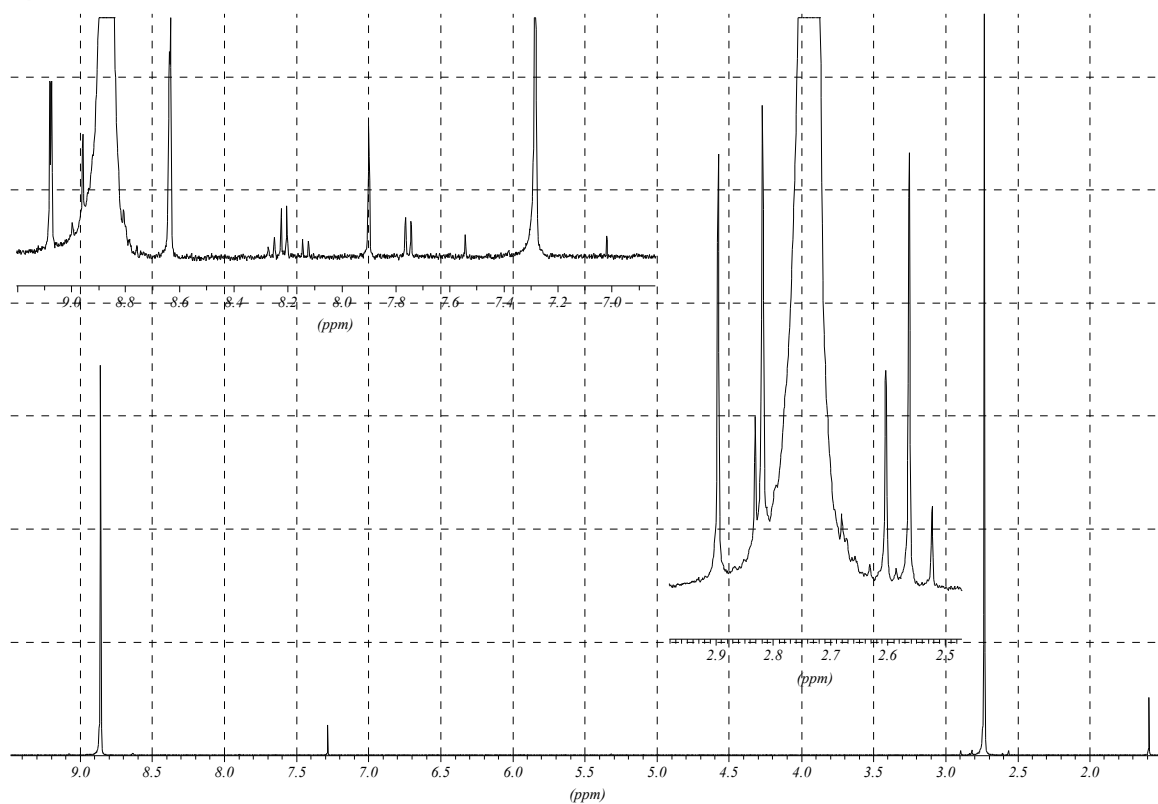
^1\text{H} NMR of Trinitrotoluene Sample
