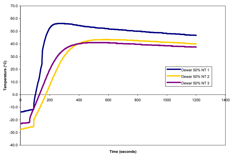
Figure 8: Addition of 50% wt./wt. nitrotoluene in DCM to concentrated \text{HNO}_3
