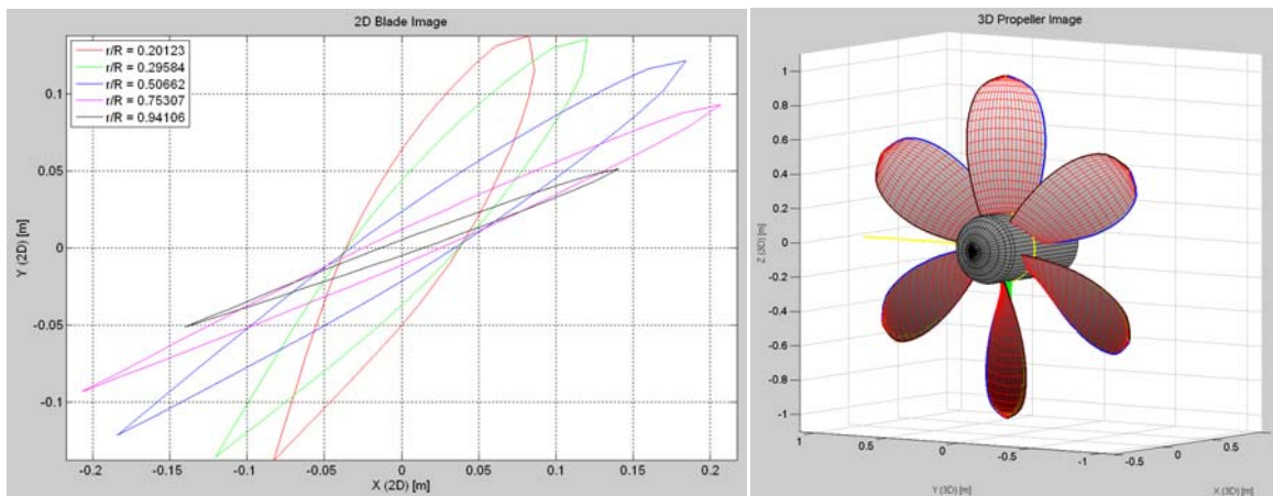
Figure 2-5: Blade and propeller representations from OpenProp
