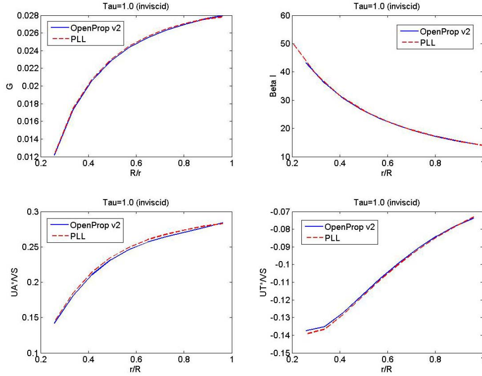
Figure 4-10: OpenProp v2 comparison with PLL for \tau = 1.0
