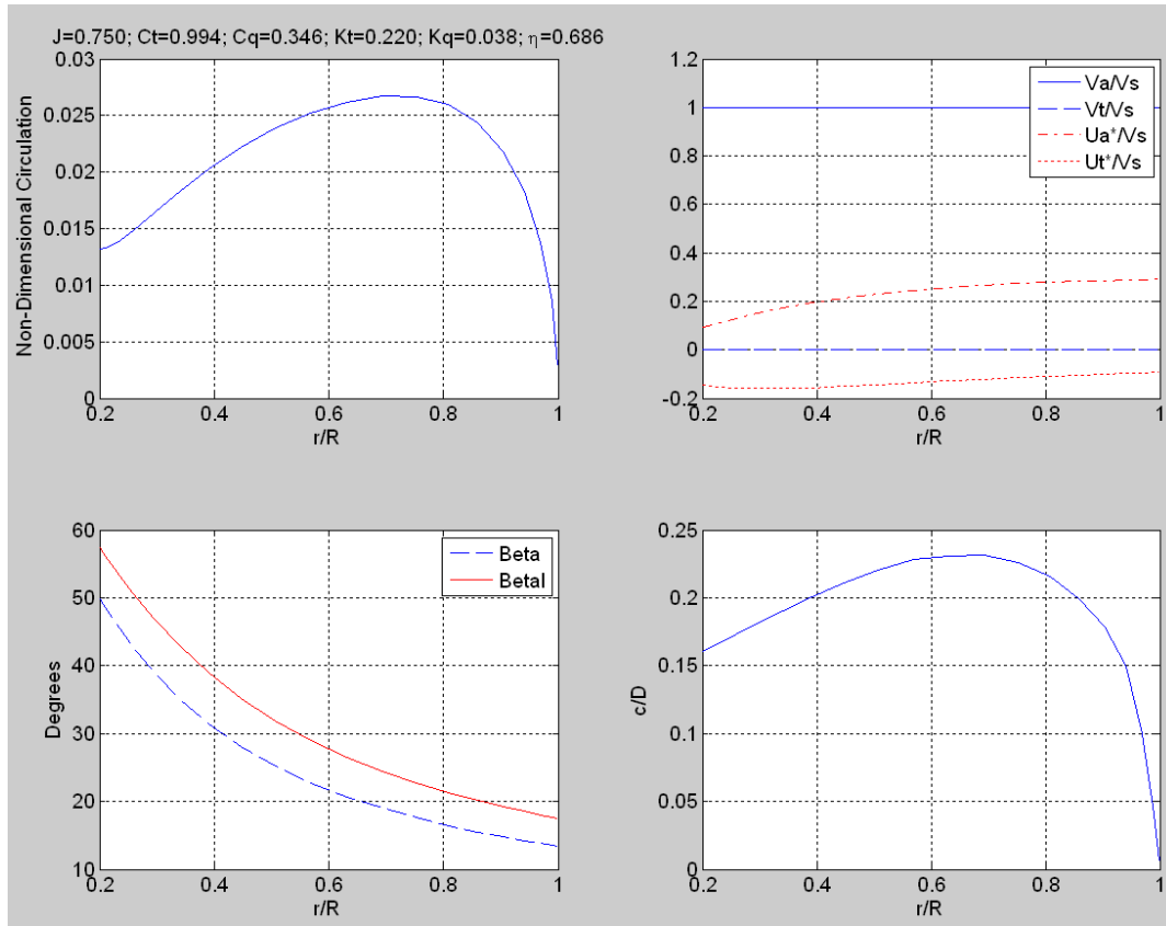
Figure 2-4: OpenProp's graphical out of key propeller parameters
