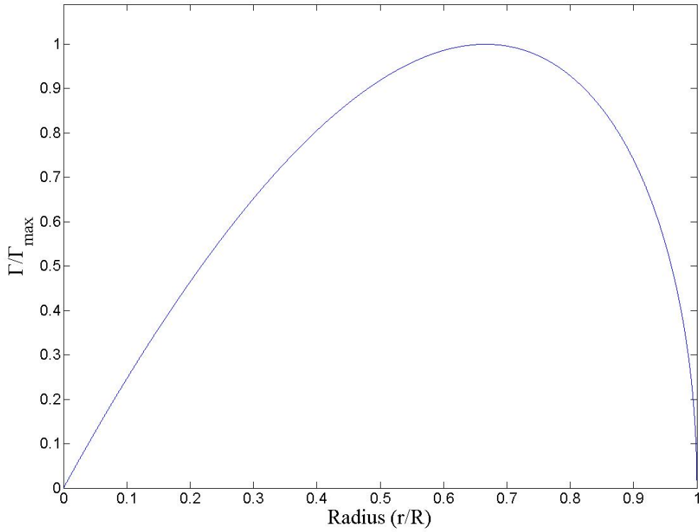
Figure 3-4: CMV.m Validation Representative Circulation
