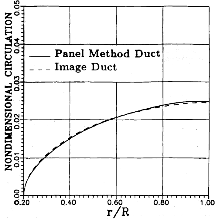
Figure 3-3: Optimization circulation distribution for a zero gap ducted propeller as determined from image and panel representations of the duct from Coney (1).
