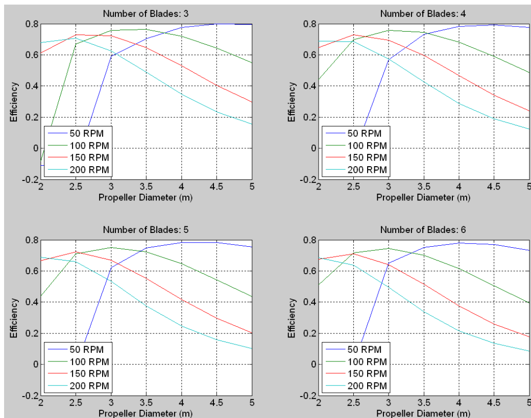
Figure 2-2: Efficiency diagrams produced by OpenProp's parametric analysis
