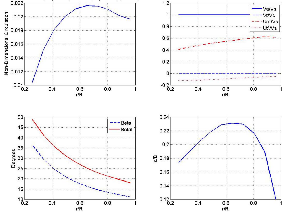
Figure 4-7: OpenProp v2 graphical output for test case with \tau = 0.8
