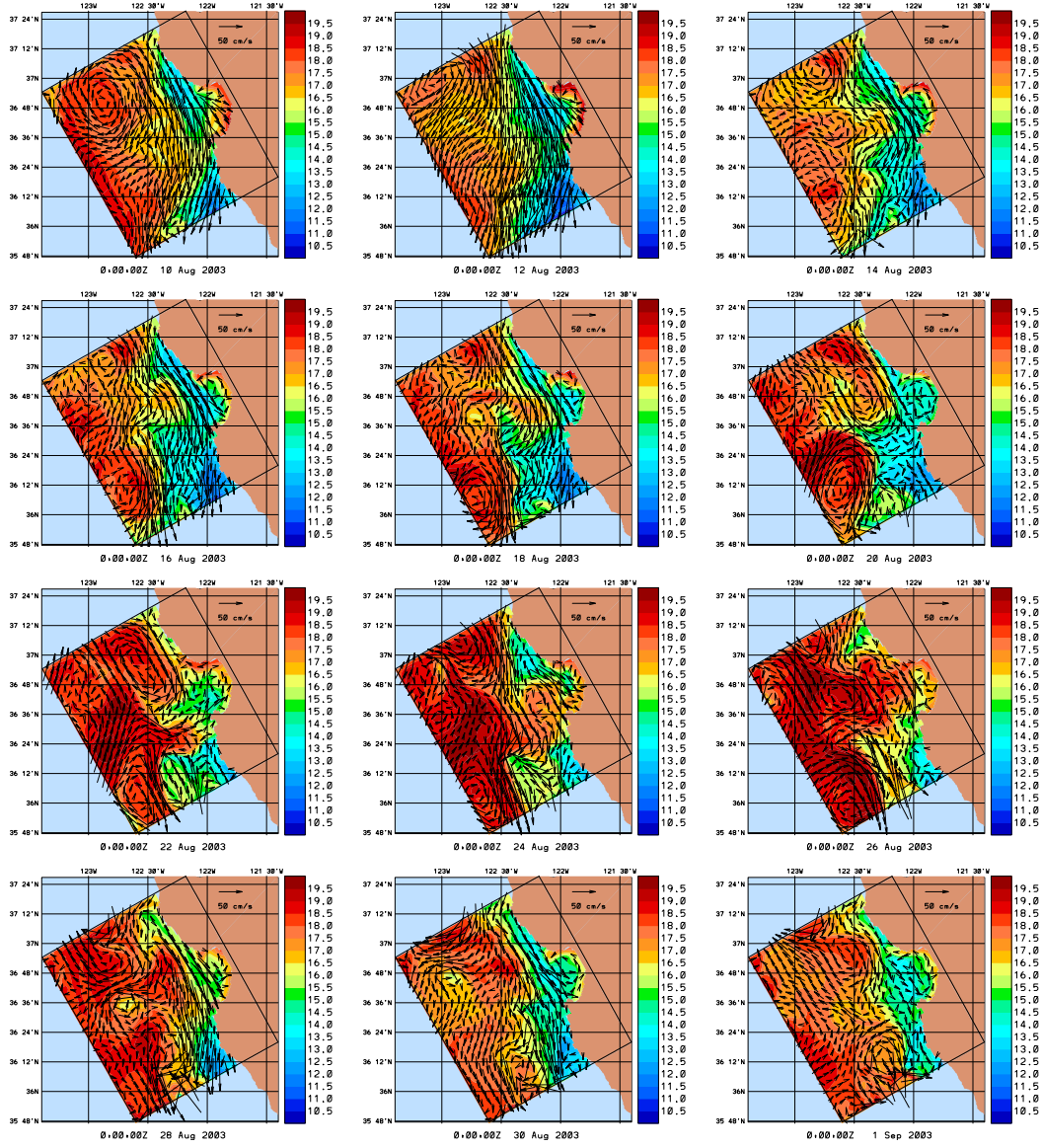
Fig. 13. Reanalysis surface temperature ( ^{\circ}\text{C} ) and velocity ( \text{cm/s} ) every 2 days for the period 10 Aug - 1 Sep, 2003.
