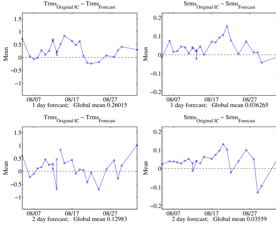
Fig. 9. Real-time volume-averaged RMS error differences. Persistence RMS - Forecast RMS, a positive result indicates skill. The left column shows results for temperature ( ^{\circ}\text{C} ), the right for salinity (PSU). The top row shows results for 1 day forecasts, the bottom row for 2 day forecasts.
