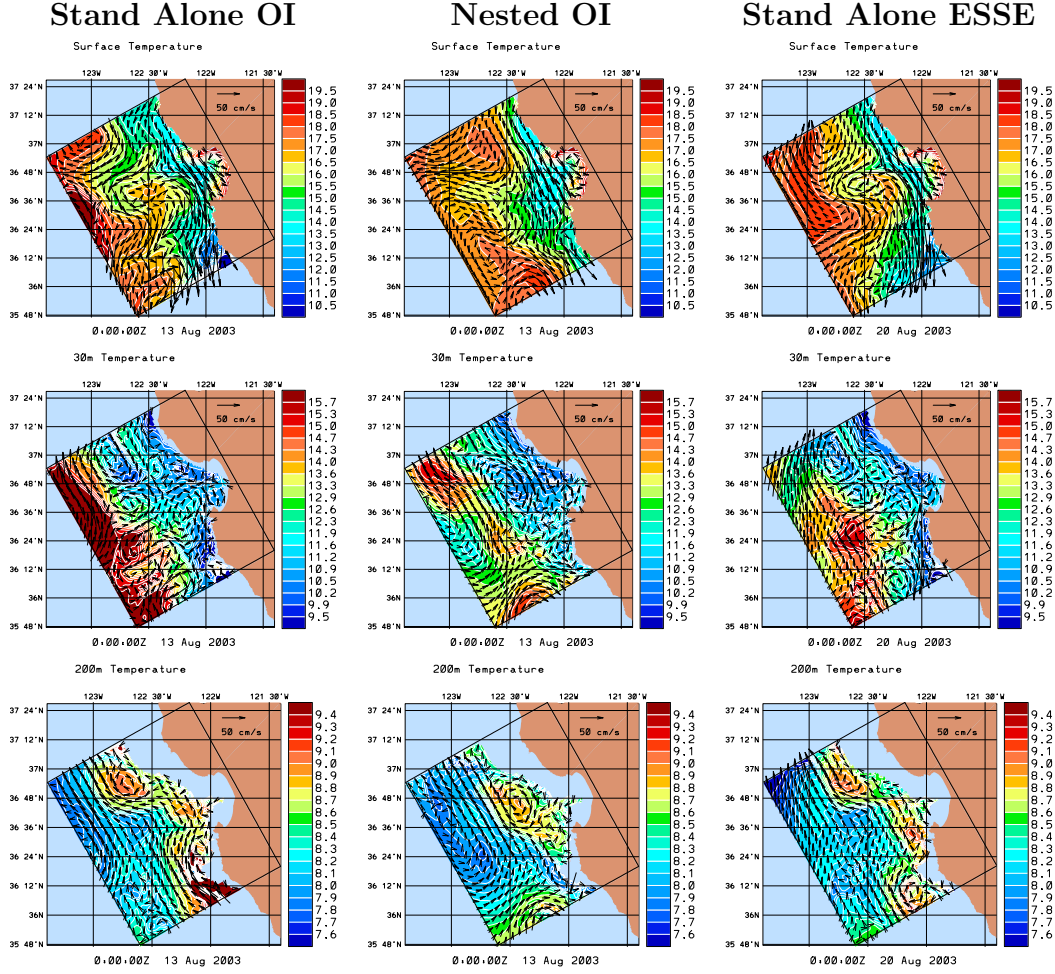
Fig. 6. Comparison of temperature ( ^{\circ}\text{C} ) and velocity ( \text{cm/s} ) for stand-alone, nested and ESSE forecasts for 13 Aug 2003.
