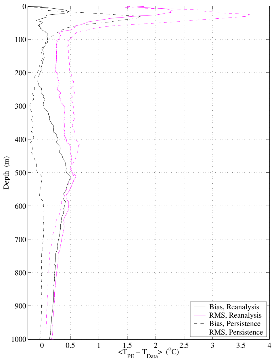
Fig. 16. Reanalysis Temperature Bias ( ^{\circ}\text{C} ) and RMS ( ^{\circ}\text{C} ) comparisons, averaged over Aug 21-25. In this reanalysis simulation, only data up to Aug 20 was assimilated. Persistence is defined as the Aug 20 objective analysis of all data up to Aug 20.
