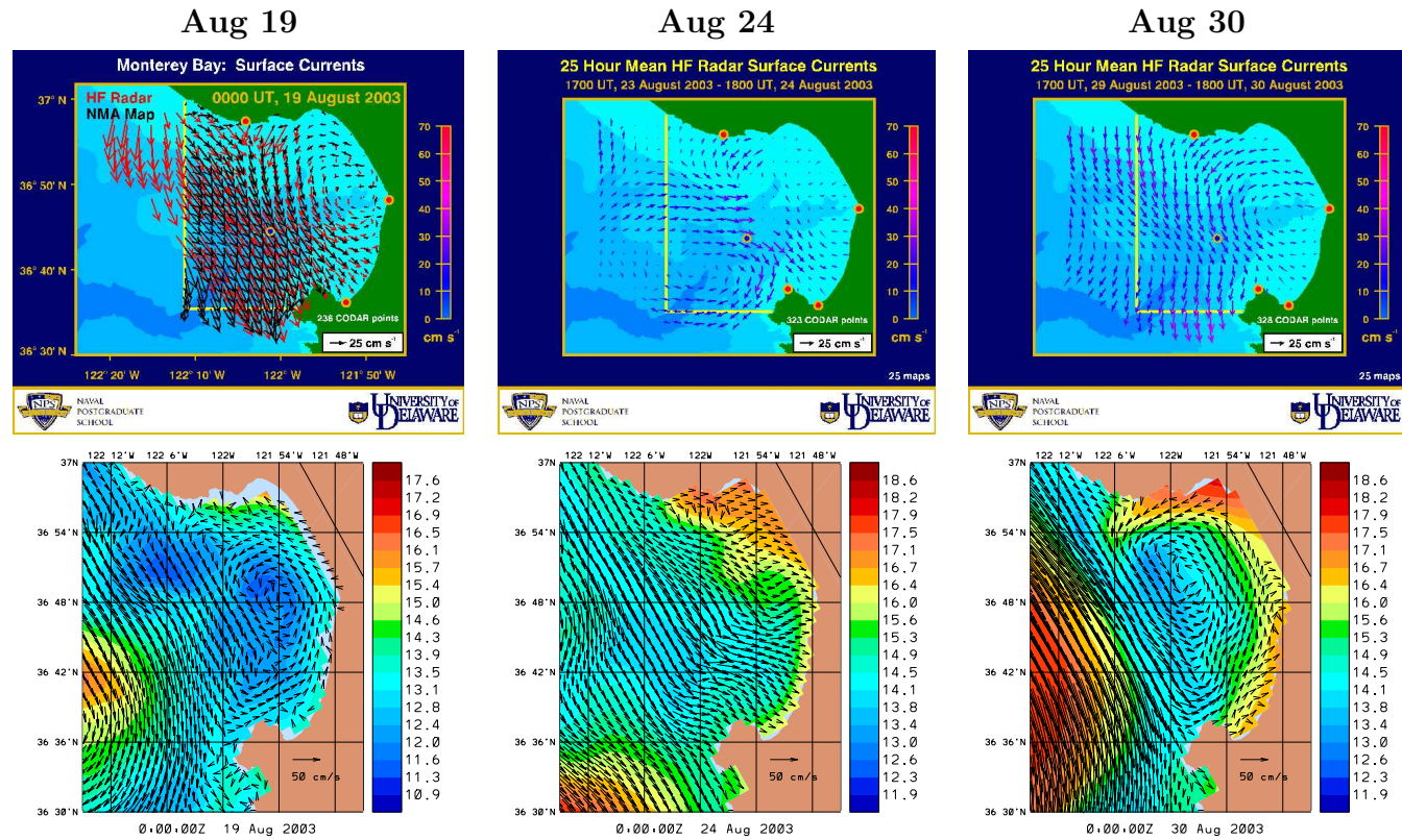
Fig. 8. Comparisons of (top row) available real-time CODAR ( \text{cm/s} ) images with (bottom row) corresponding real-time forecast surface velocity ( \text{cm/s} ) fields.
