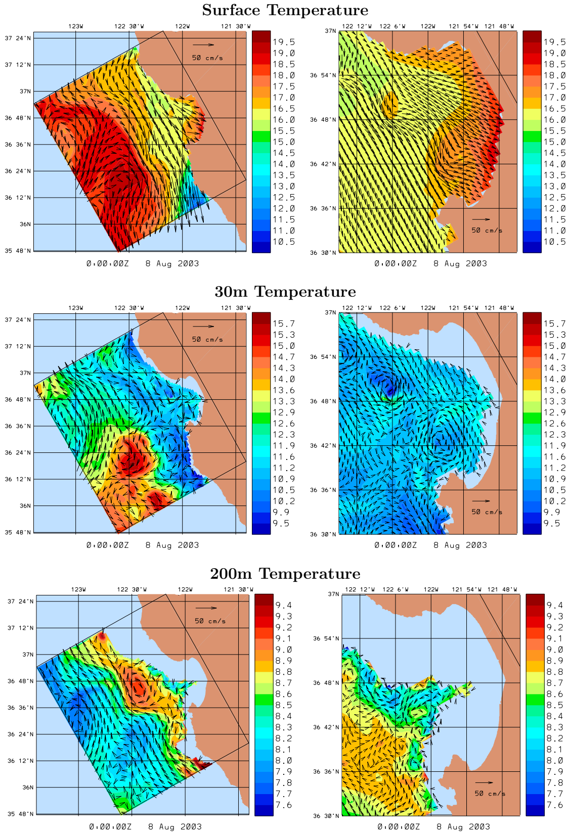
Fig. 5. Temperature ( ^{\circ}\text{C} ) and velocity ( \text{cm/s} ) fields for Aug 8, 2003 issued during the real-time exercise. These fields show the general structures that were observed in real-time.
