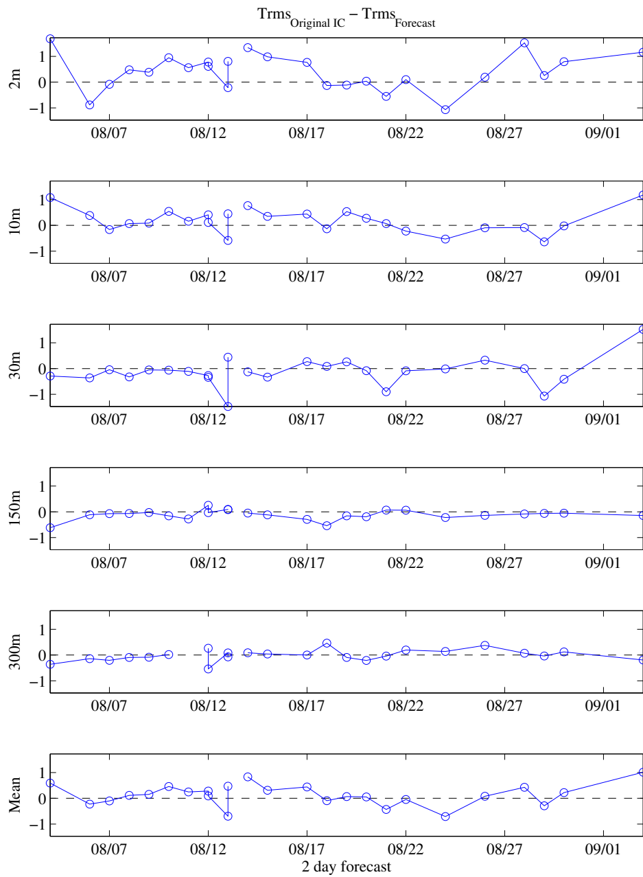
Fig. 11. Real-time Temperature RMS differences ( ^{\circ}\text{C} ) for 2 day forecasts. Persistence RMS - Forecast RMS, a positive result indicates skill.
