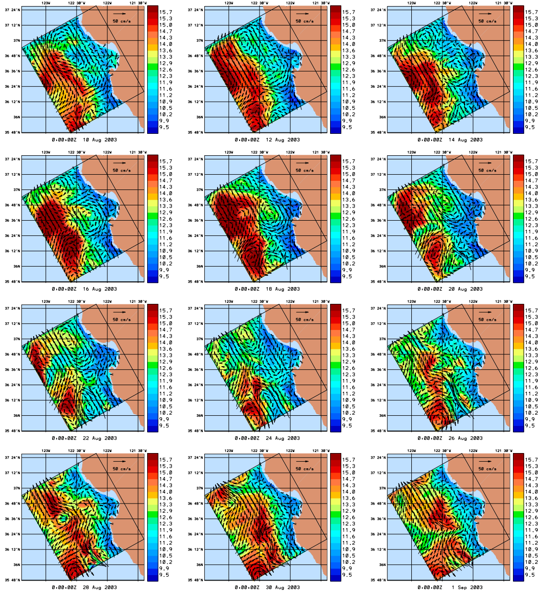
Fig. 14. Reanalysis 30m temperature ( ^{\circ}\text{C} ) and velocity ( \text{cm/s} ) every 2 days for the period 10 Aug - 1 Sep, 2003.
