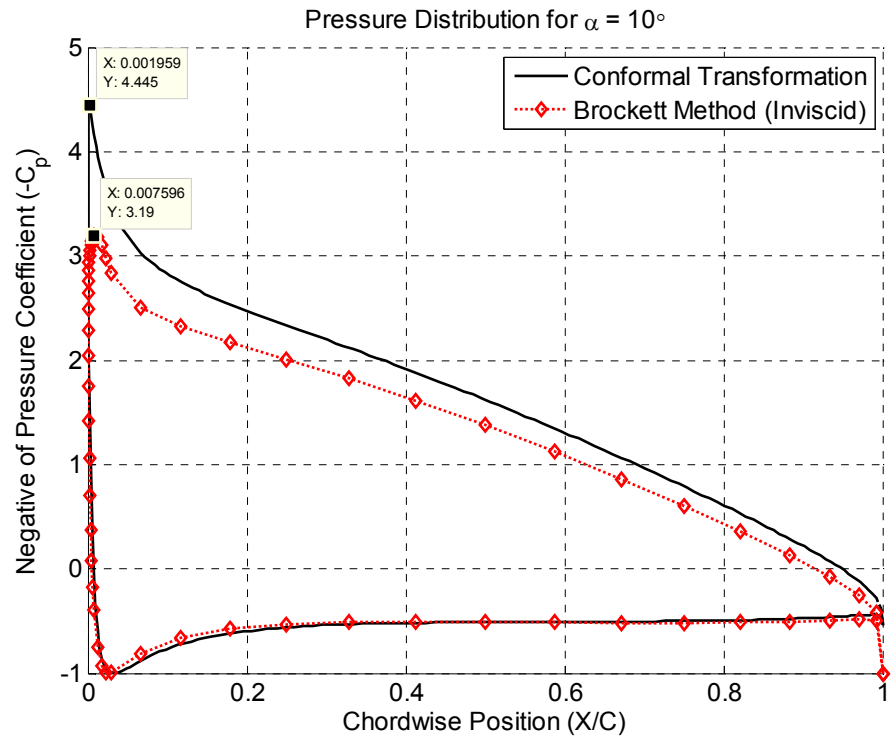
Figure 6: Comparison of Brockett Method to Exact Solution, \alpha = 10^\circ
