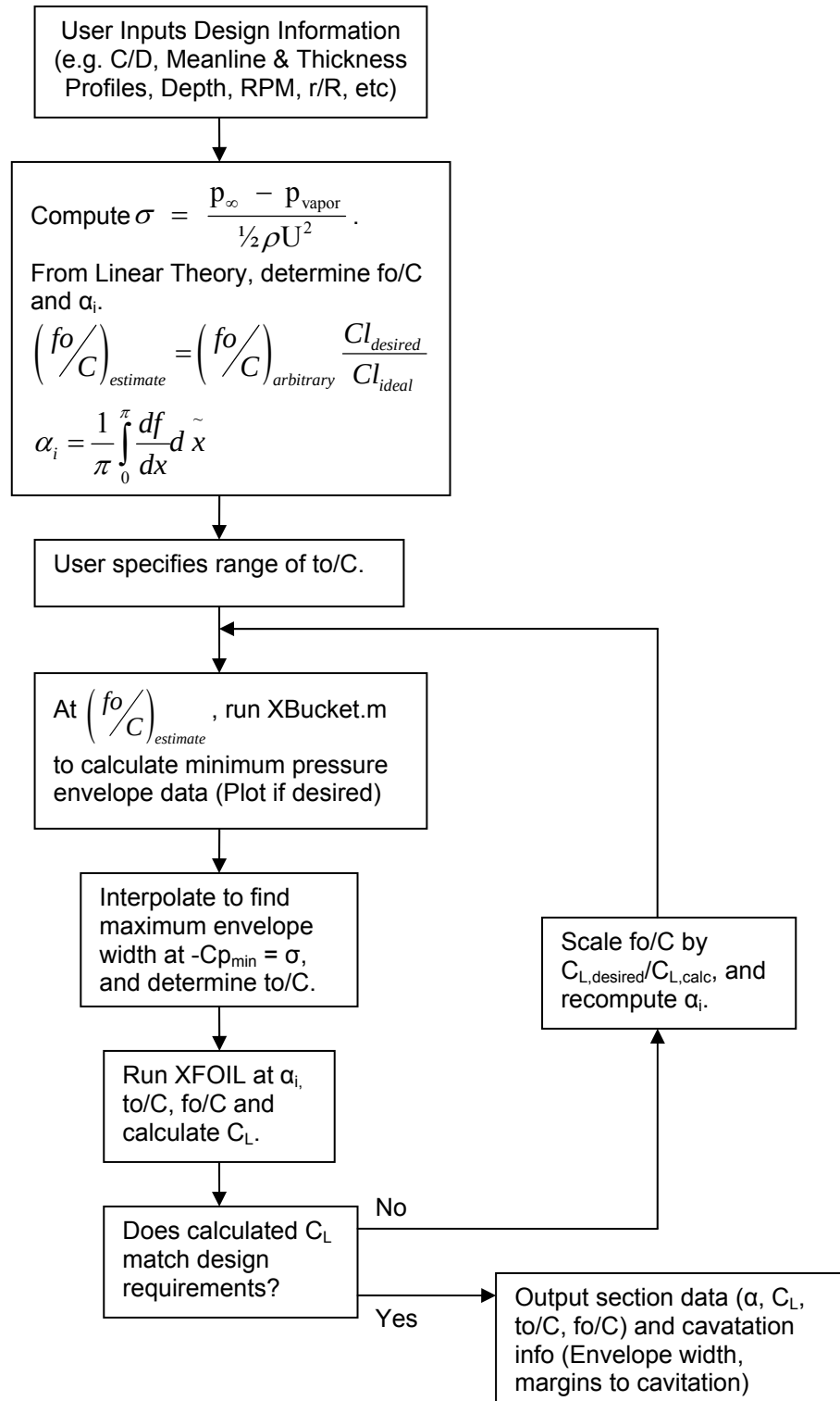
Figure 17: Example Flowchart for using Minimum Pressure Envelopes for Design.
