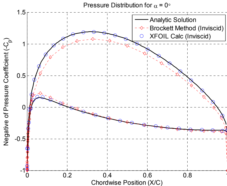
Figure 8: Comparison of XFOIL and Brockett Method to Exact Solution, \alpha = 0^\circ
