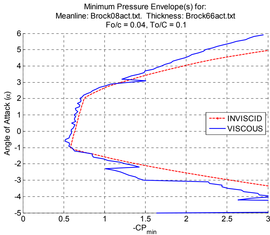
Figure 14: Sample Viscous and Inviscid Minimum Pressure Envelopes Calculated by XFOIL (Reynolds Number = 1 \times 10^6 , 100 Maximum Iterations)
