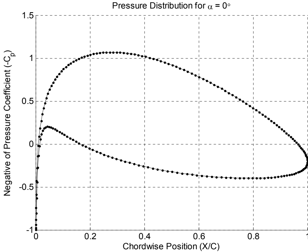
Figure 3: Karman-Trefftz Foil Pressure Distribution.
