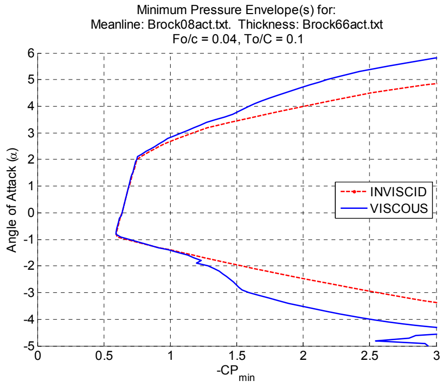
Figure 15: Sample Viscous and Inviscid Minimum Pressure Envelopes Calculated by XFOIL (Reynolds Number = 1 \times 10^6 , 100 Maximum Iterations, 70 Panels)
