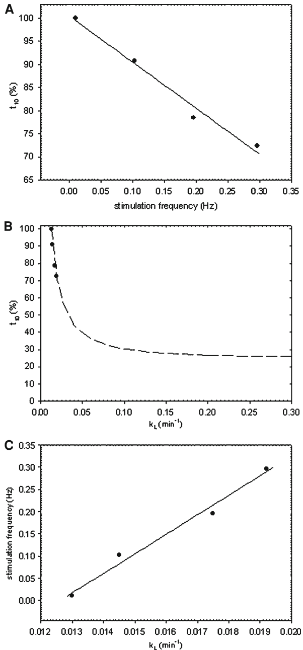
Fig. 2 Different values of k_L in the 3-step model simulated the frequency-dependence of the rate of onset of BoNT/A-induced paralytic activity. Panel A: plot of data points where values for t_{10} are expressed as normalized values. Panel B: The 3-step model (dashed line) produced a non-linear relation between k_L ( 0.01 - 0.3 \text{ min}^{-1} ) and the time-to-10% tension, t_{10} . Within the range of experimental data, the plot was linear and at higher values of k_L approached an asymptotic value for the normalized values of t_{10} . Panel C: Values of k_L were adjusted to simulate normalized t_{10} values at each of the four experimentally used nerve stimulation frequencies. Circles: experimental data from Fig. 4 in [15]; lines in Panels A and C: least-squares fits drawn through the data points
