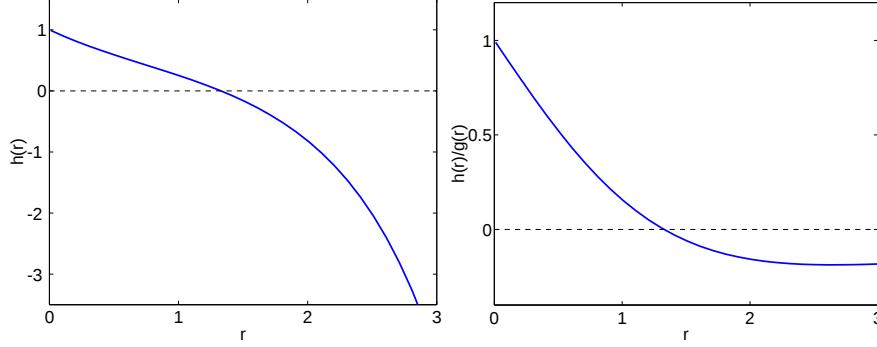
FIG. 3.1. Graphs of functions h(r) and \frac{h(r)}{g(r)} . The left panel shows the graph of function h(r) . From the graph, it is clear that h(r) is a decreasing function of r for r>0 and h(r) \rightarrow -\infty as r \rightarrow +\infty , as described in Theorem 1. h(r) intersects with the horizontal axis at r_0=1.32757384 . Function h(r) satisfies 1>h(r)>0 for r<r_0 and h(r)<0 for r>r_0 . The right panel shows the graph of function \frac{h(r)}{g(r)} .
